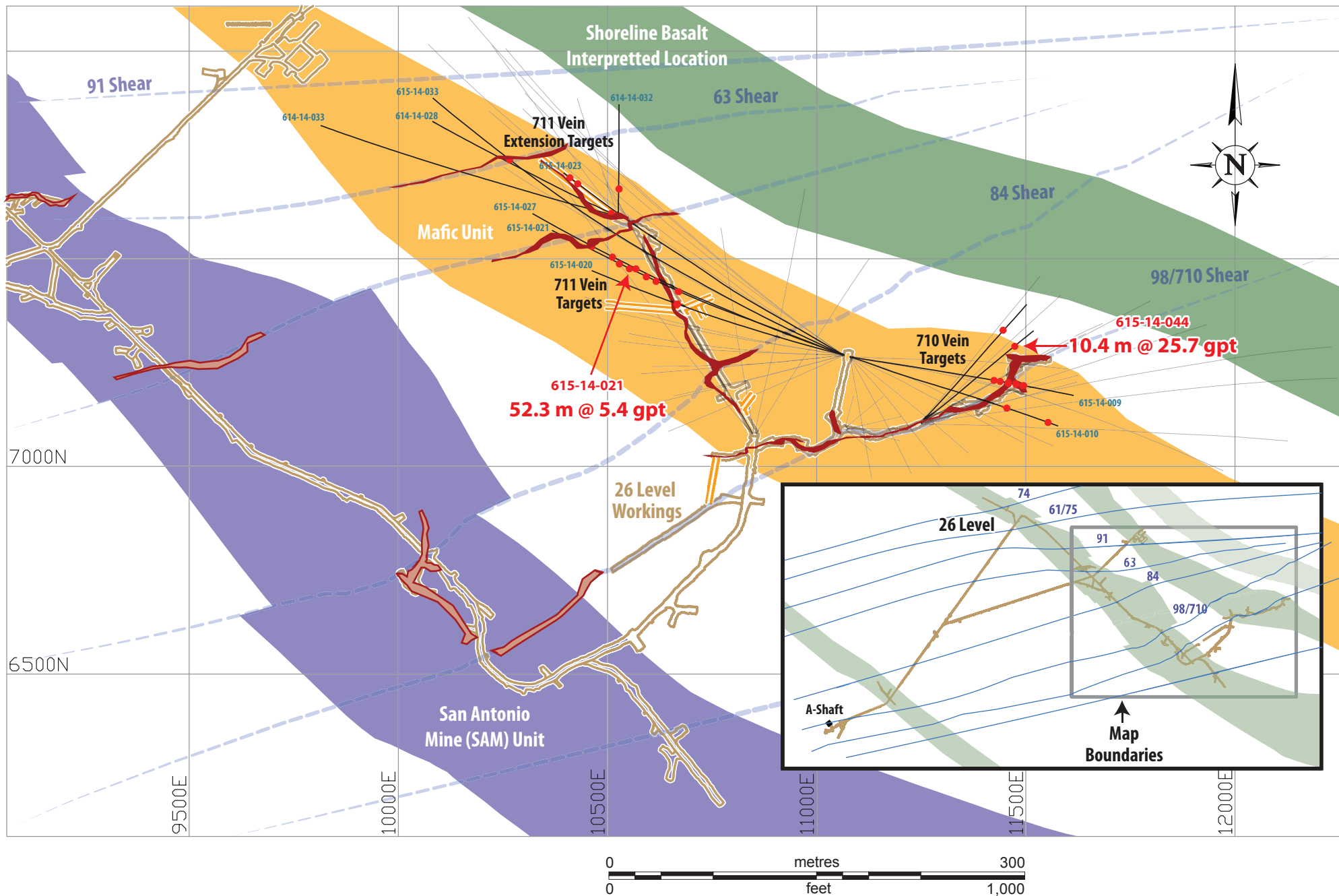
Figure 1: 26 Level Plan View of Drilling, Shears and Structures - Rice Lake Mine
