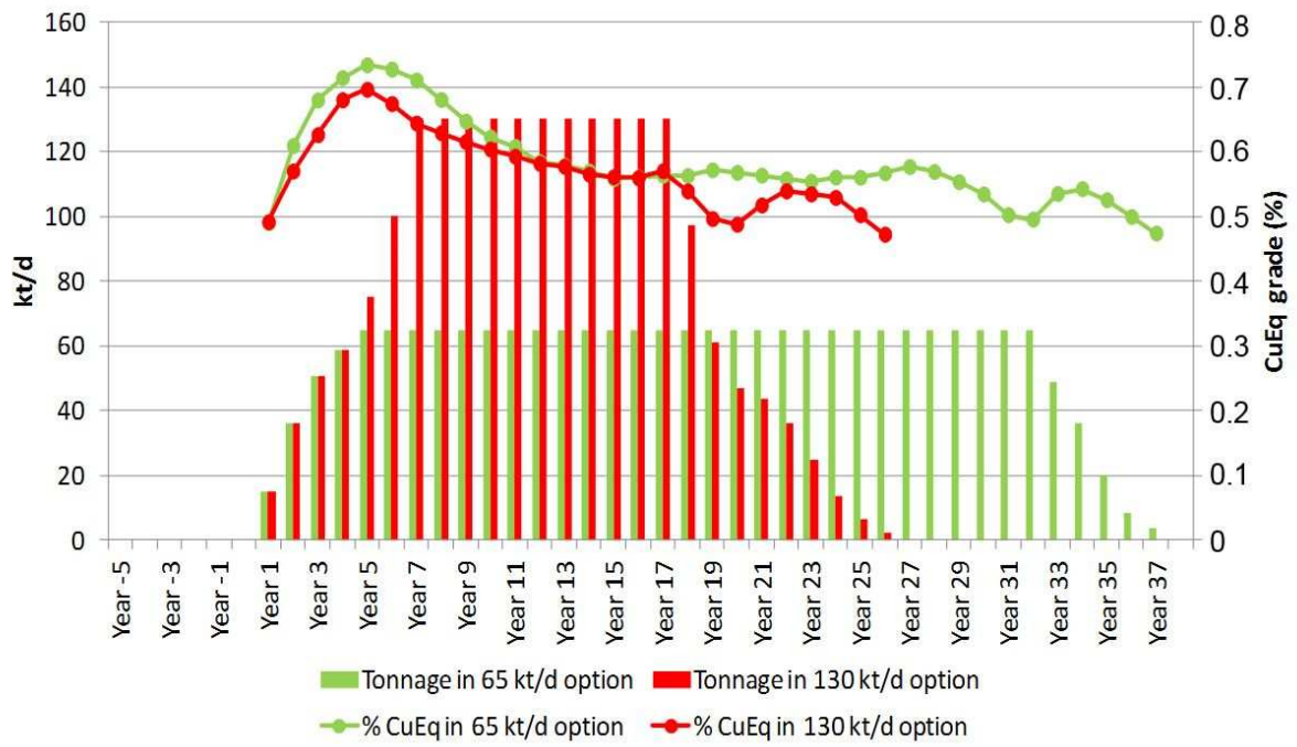
Production Programs 65 & 130 kt/d Options
