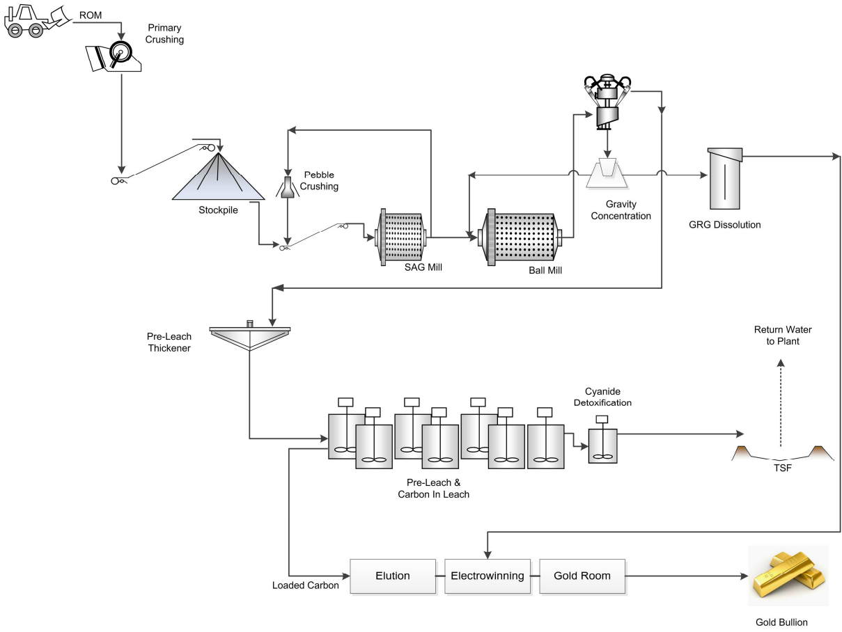
Figure 2: Process Flow Sheet
