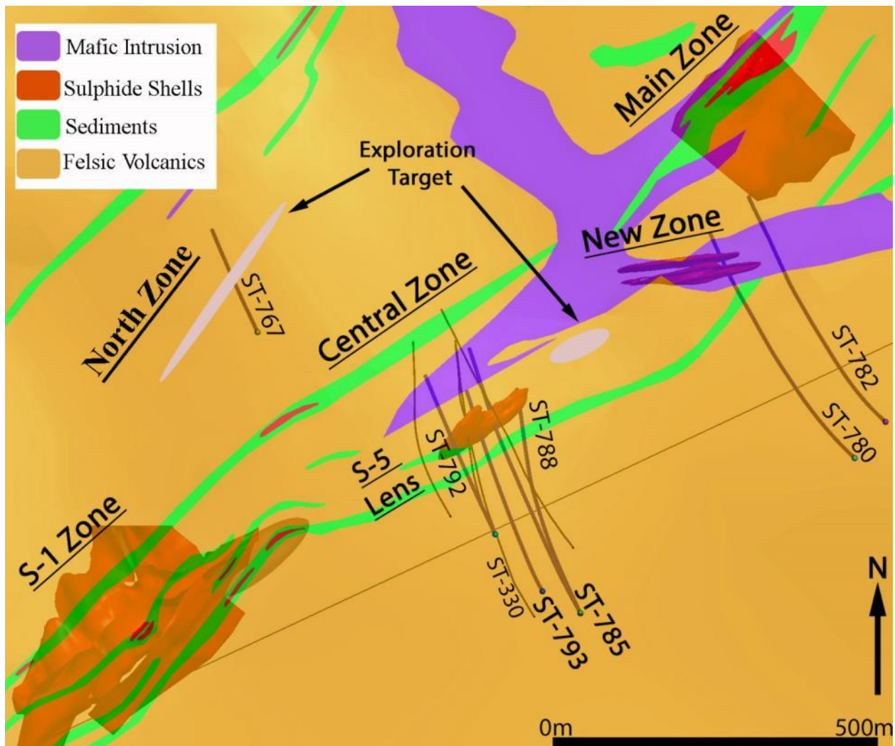
Figure 1: Geology map with 3-D projection of mineralization
