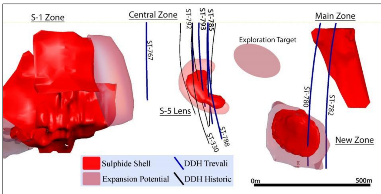
Figure 2: 3D Long section view of the Stratmat Deposits Looking N333°
