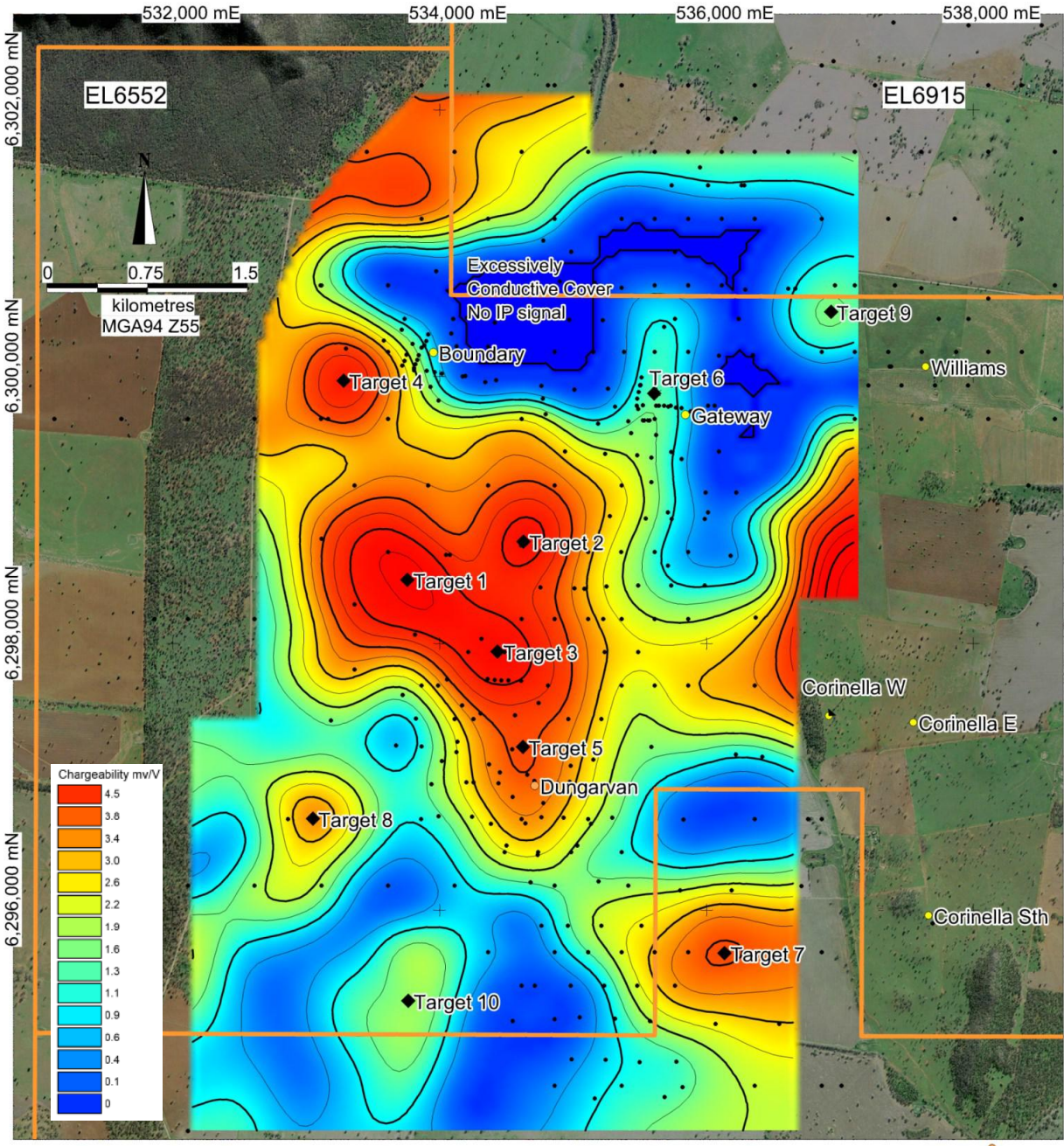
Figure 1: Plan view of the 3D chargeability model sliced at -450-metre depth, showing the locations of the 10 targets (contoured at 0.5mV/V intervals) with respect to the drill collars and prospect locations.
