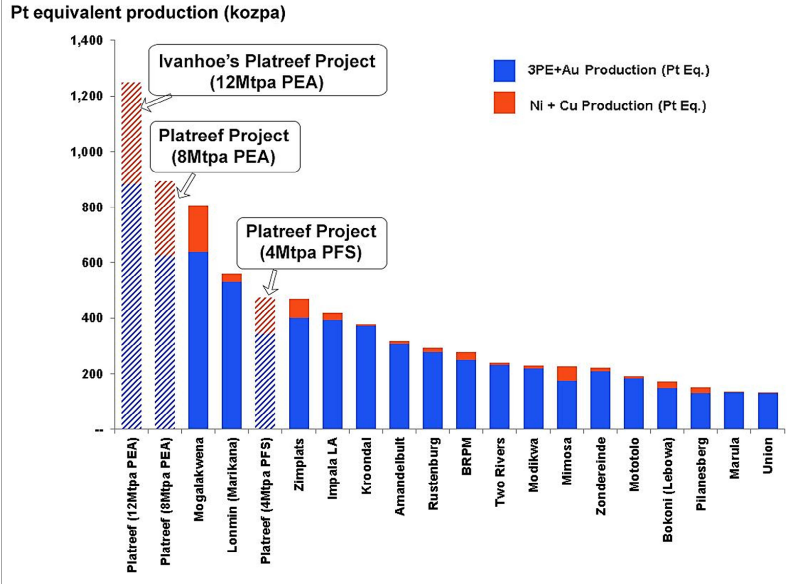
Figure 2.0: Total 2014E platinum equivalent production in Africa.
