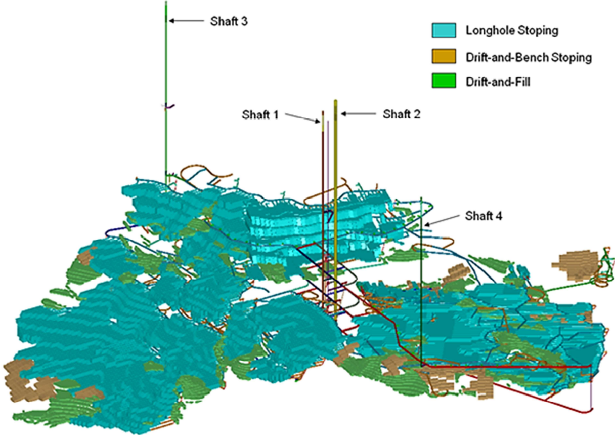
Figure 3.0: Elevated view of mining areas by method (isometric view).
