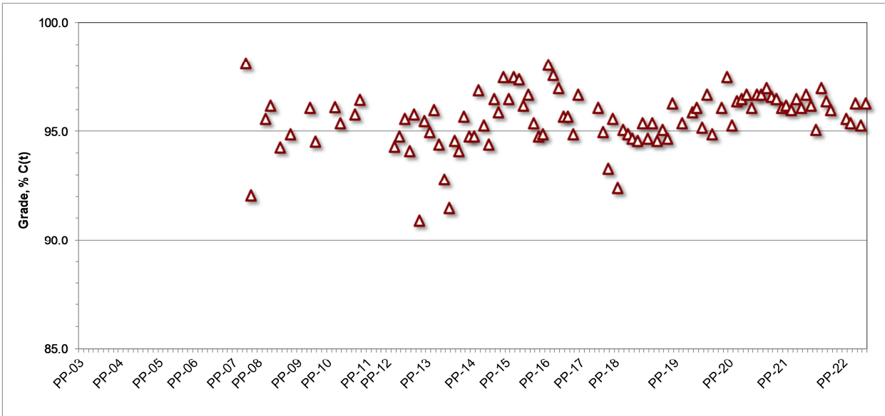
Figure 3: Combined (Final) Concentrate Grade from Grab Samples
