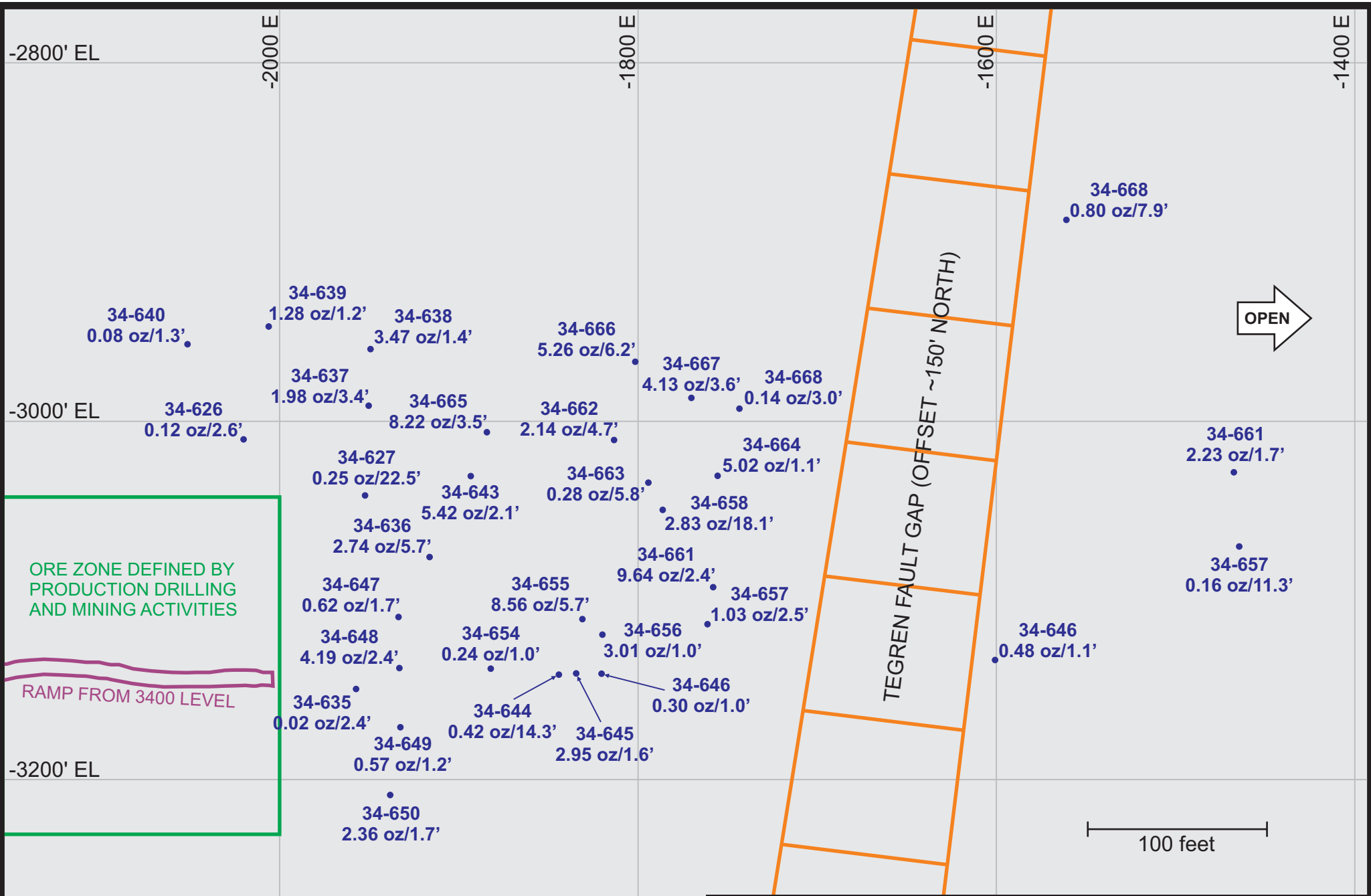
FIGURE 2 DETAILED LONG SECTION SHOWING THE LATEST UNDEGROUND EXPLORATION RESULTS, MACASSA MINE, KIRKLAND LAKE, ONTARIO. FEB. 23, 2015
