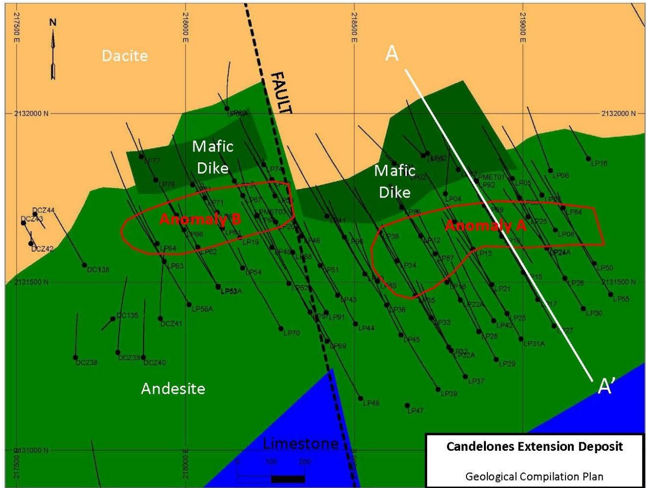
Figure 1 – Candelones Extension Geological Compilation Plan View
