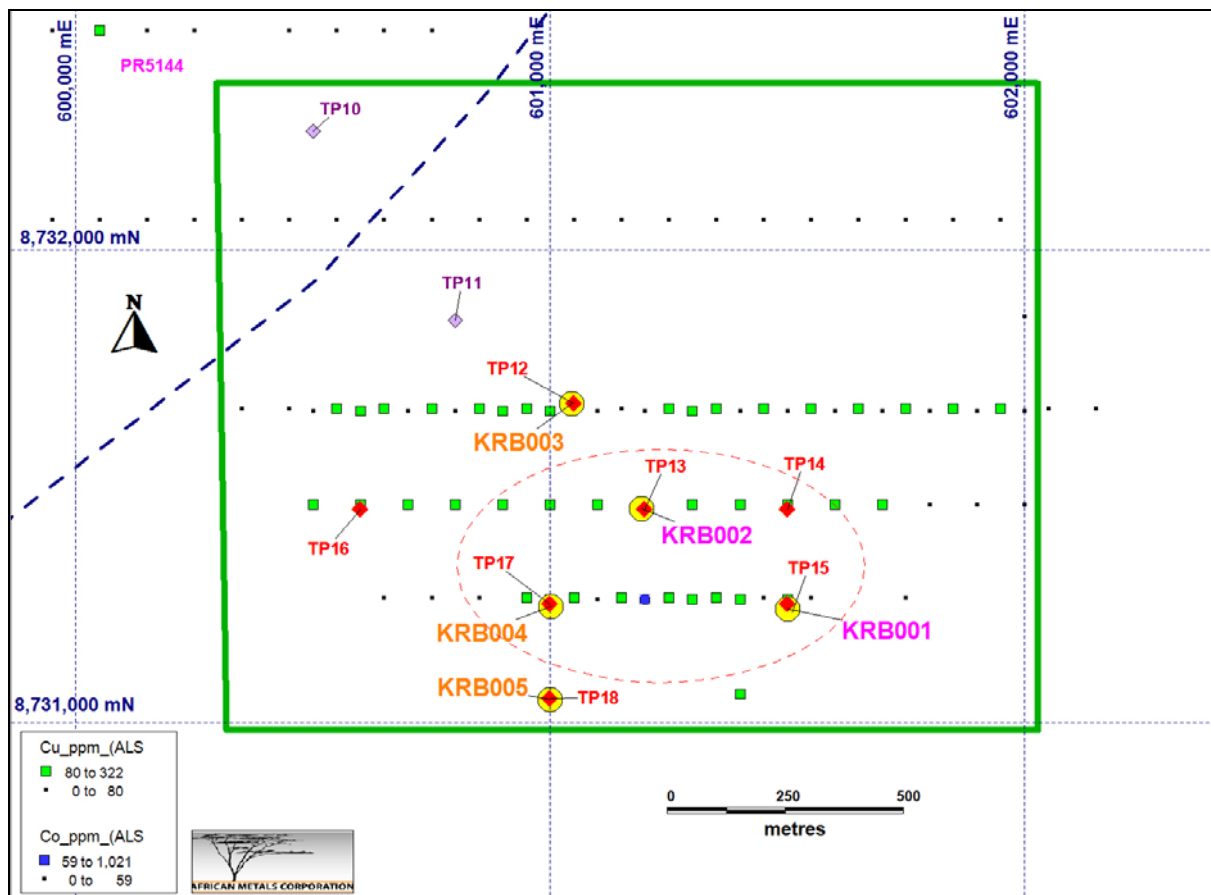
Figure 2: Kalande Project Test Pit and Drill Hole Locations – close up.
