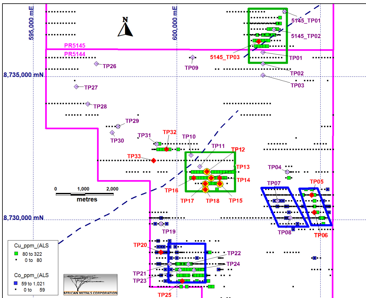
Figure 1: Kalande Project Test Pit and Drill Hole Locations
