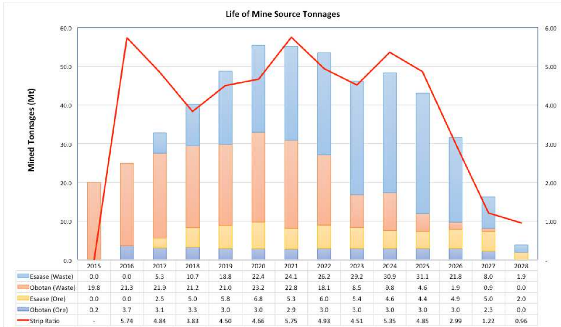
Figure 2: PFS Ore Mine Plan (un-optimized) for Asanko Gold Mine
