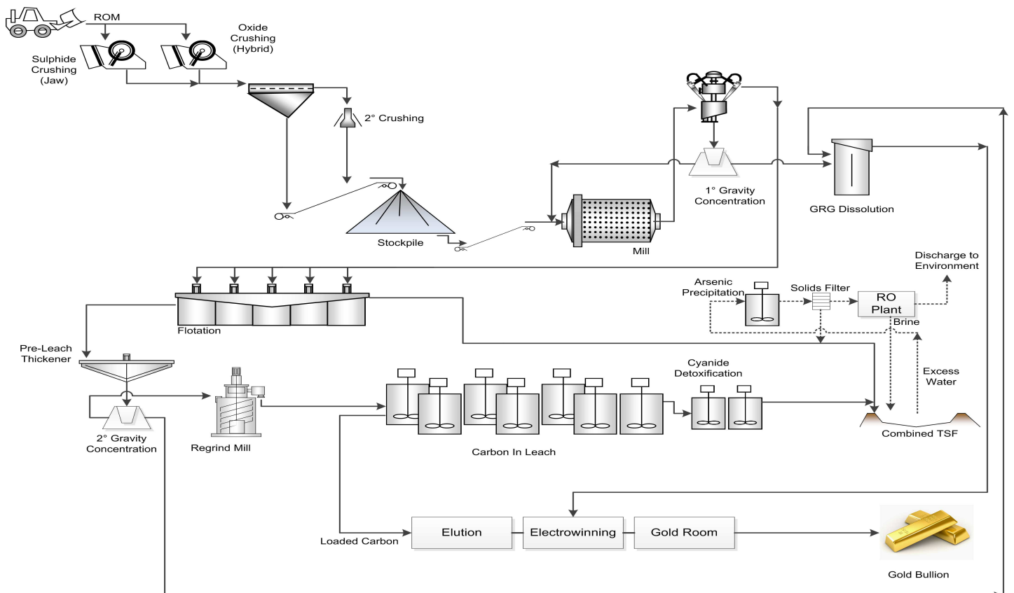
Figure 4: Phase 2 Process Flow Sheet – Addition of 5Mtpa Flotation Plant
