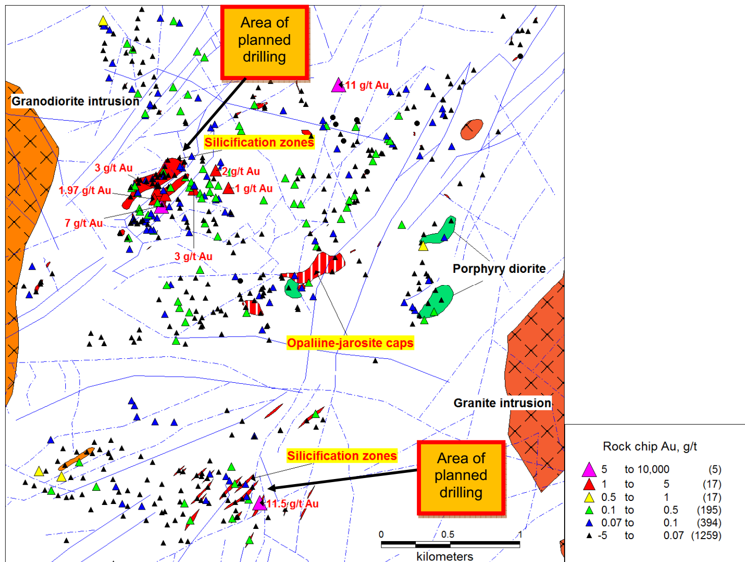
Figure 3 – Zhanatobe Central Area Geological Map with rock chip sampling results
