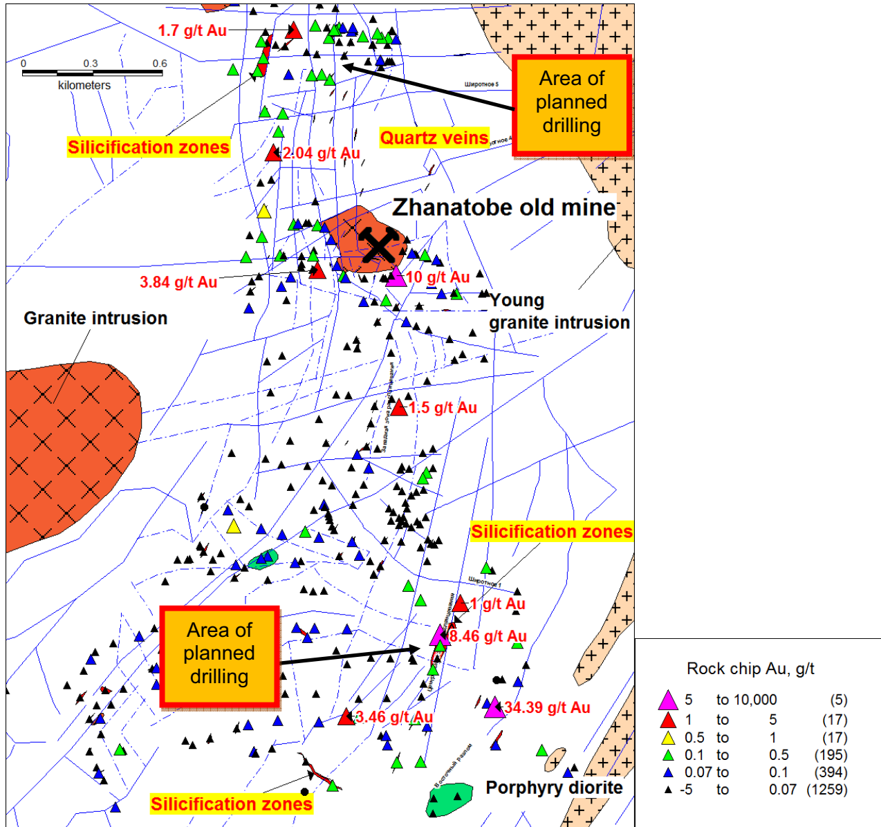
Figure 2 – Zhanatobe Northern Area Geological Map with rock chip sampling results
