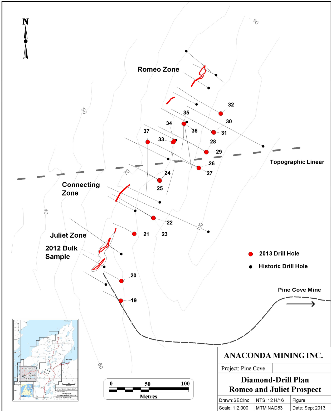
Figure 2: Romeo and Juliet Drill Plan
