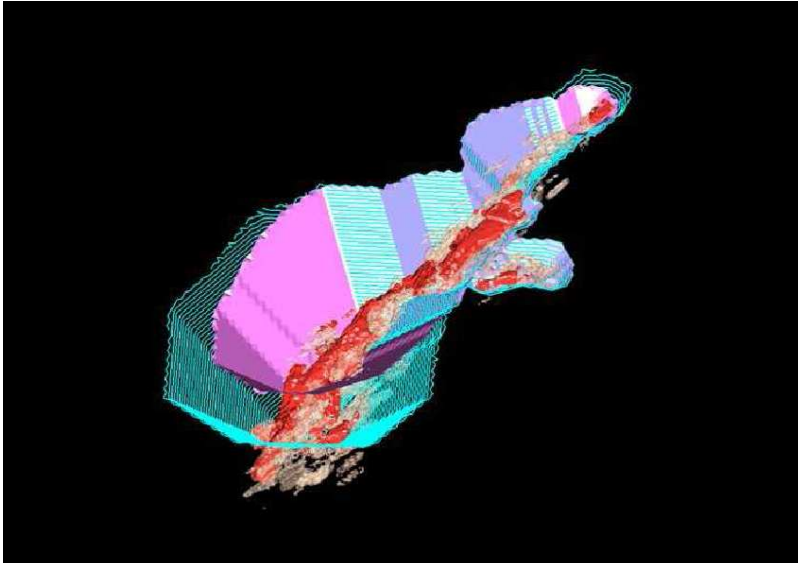
Horizontal section for bench 295 showing the outlines for both restricted and unrestricted pits.
