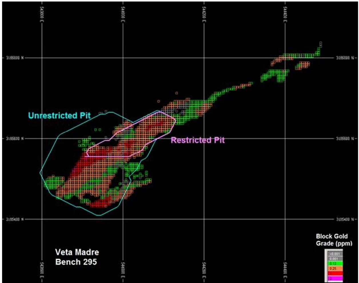
Horizontal section for bench 295 showing the outlines for both restricted and unrestricted pits.
