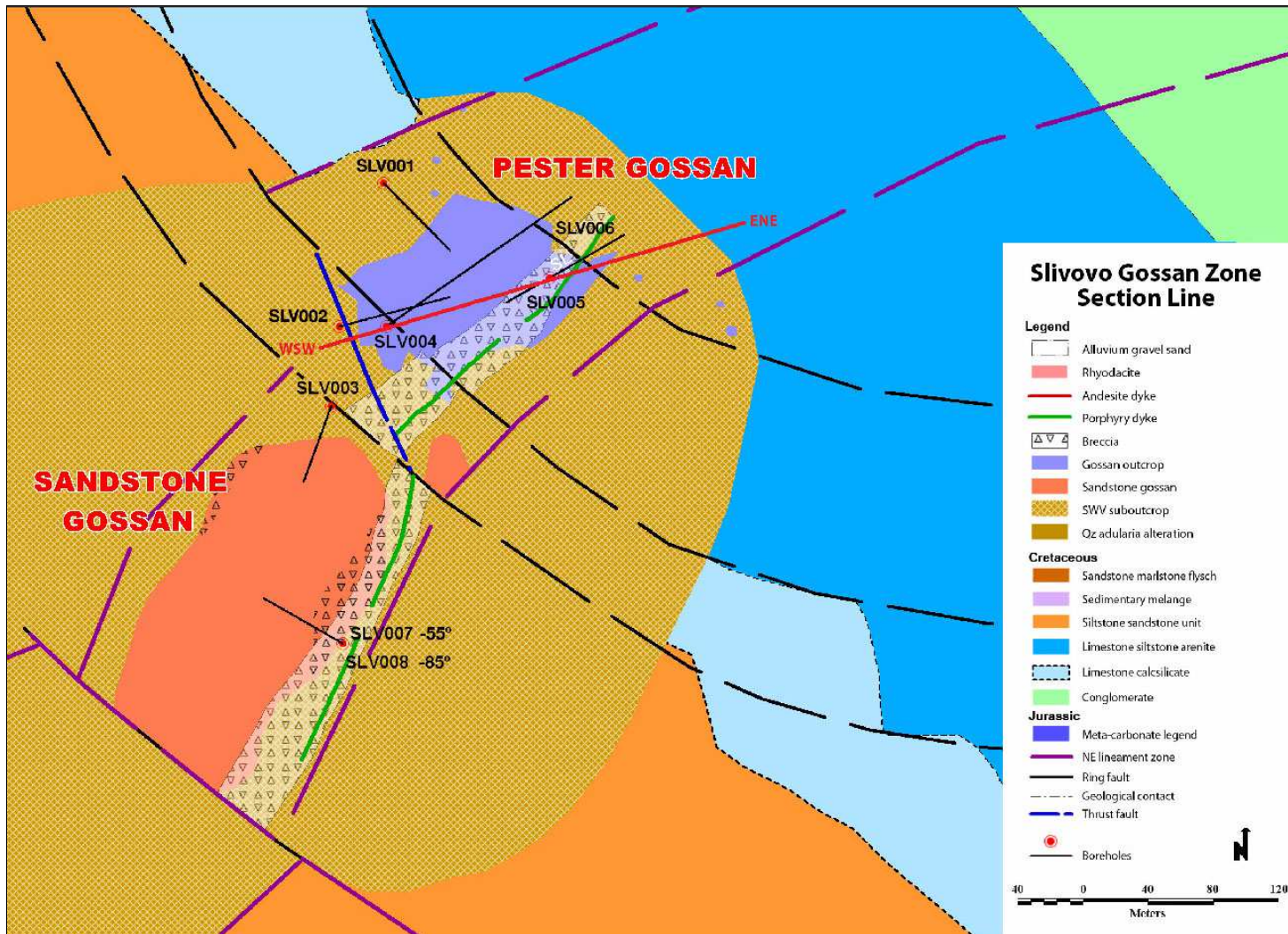
Figure 1. Plan view of gossan zone with drill hole locations and location of the Slivovo long section.
