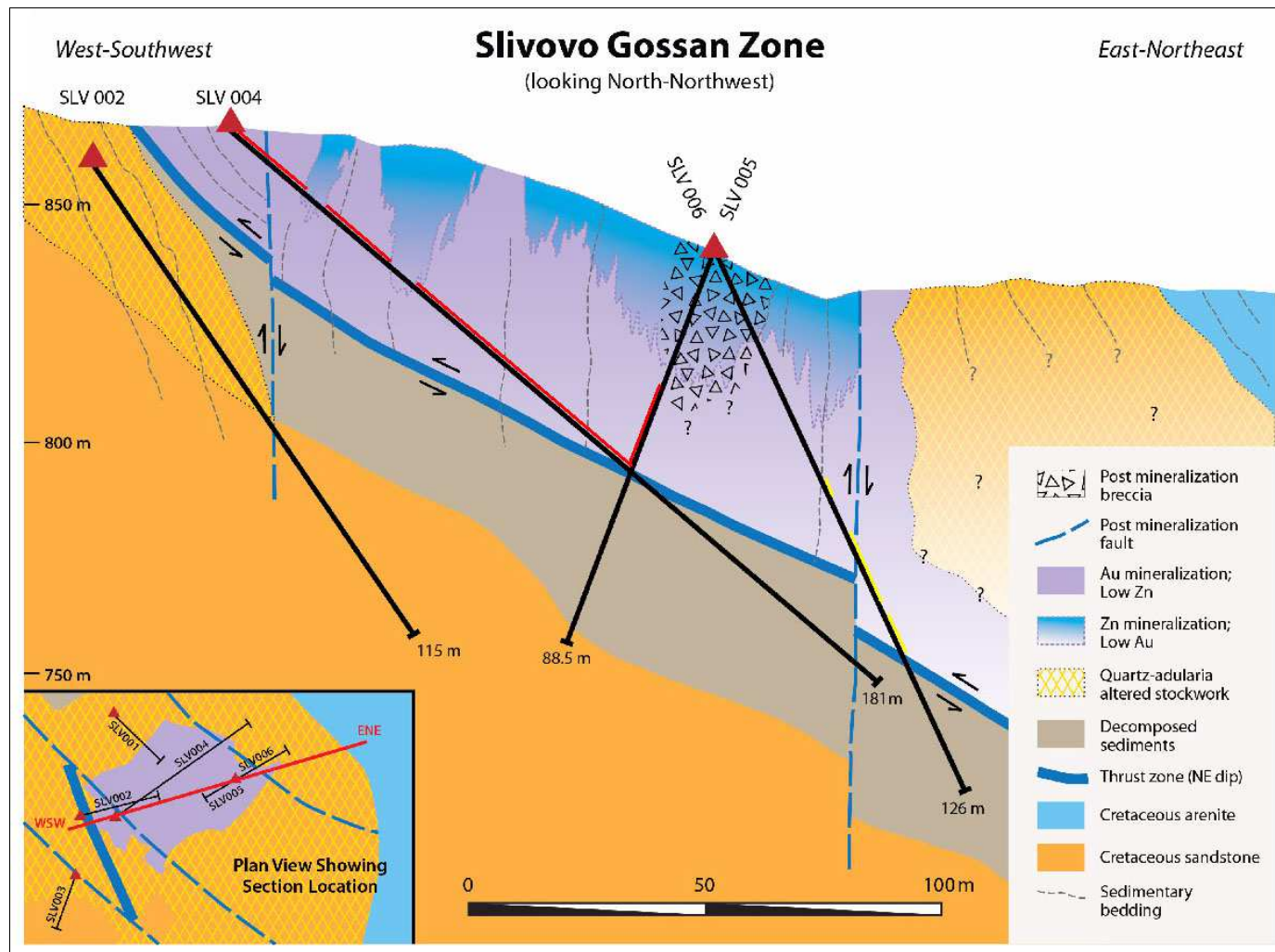
Figure 2. Schematic section showing present understanding of the prospect mineralization. Red zones along trace of the drill holes shows higher grade intercepts in SLV004 and SLV005. Yellow zones along the trace of SLV006 shows medium grade gold intercepts.
