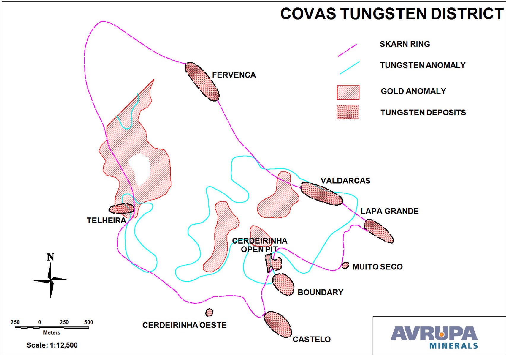
Figure 1. Gold (red) and tungsten (turquoise) anomalies in the Covas Dome
