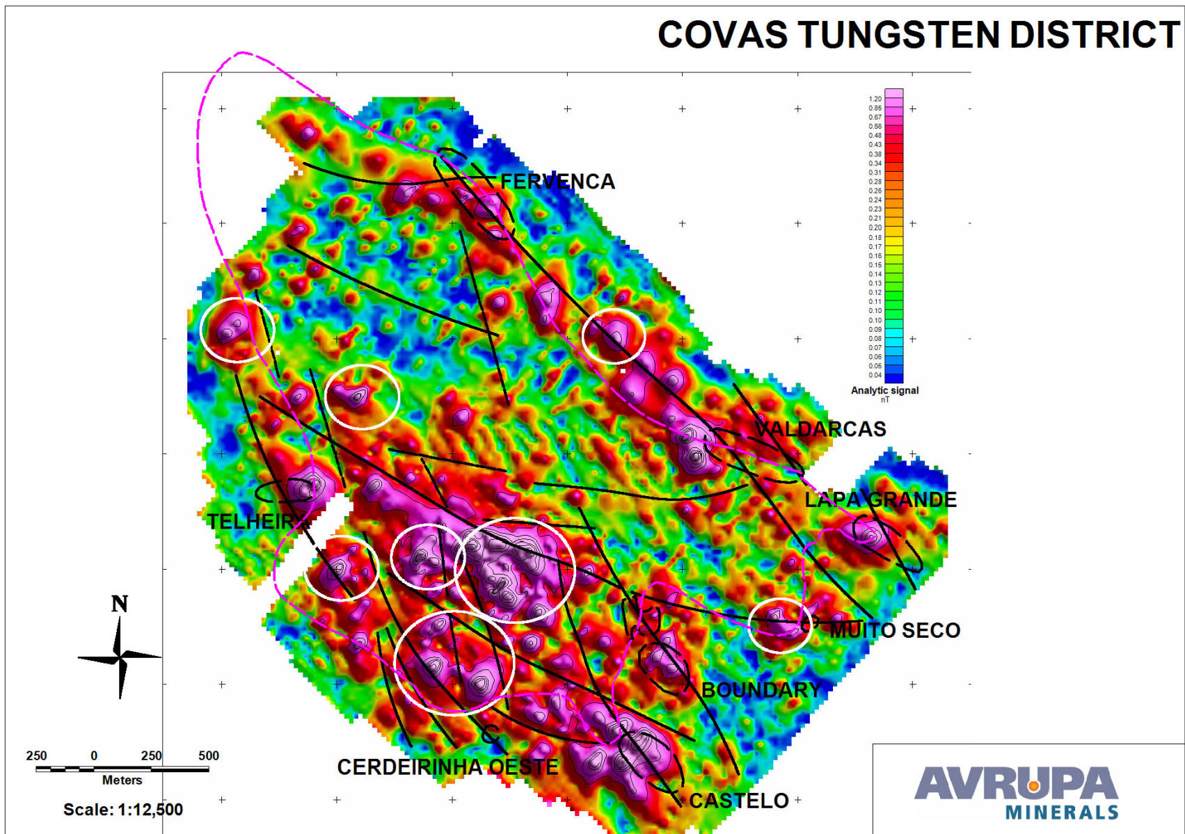
Figure 2. New magnetic anomalies (white ovals) at Covas. Note anomalism around the Skarn Ring (purple dashed).
