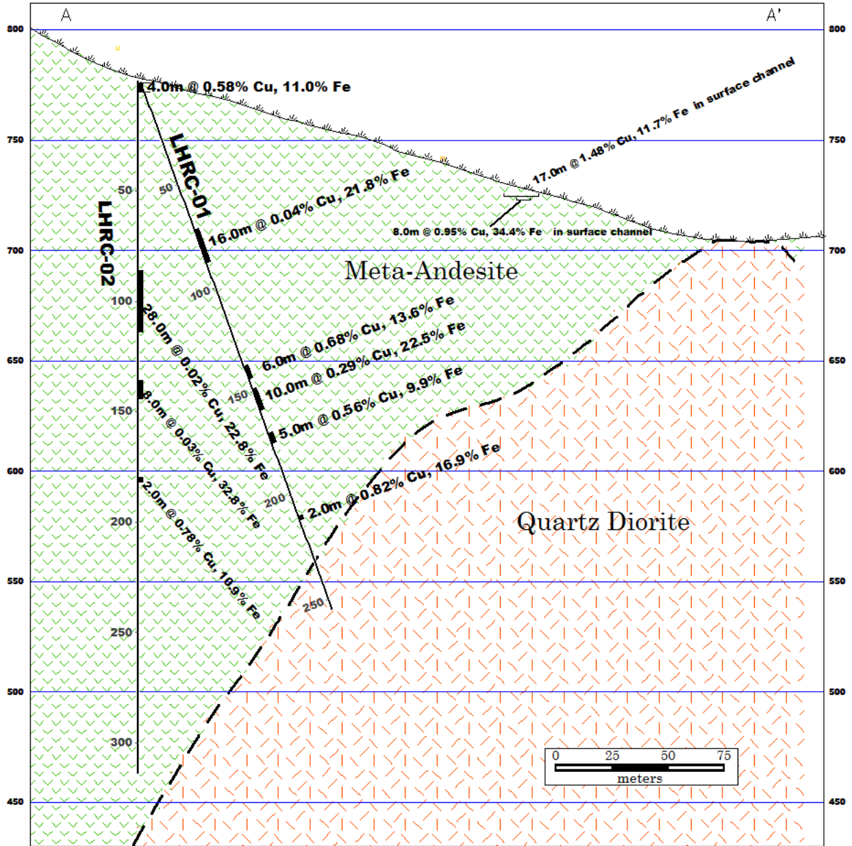
FIGURE 2 DRILL SECTION A-A'
