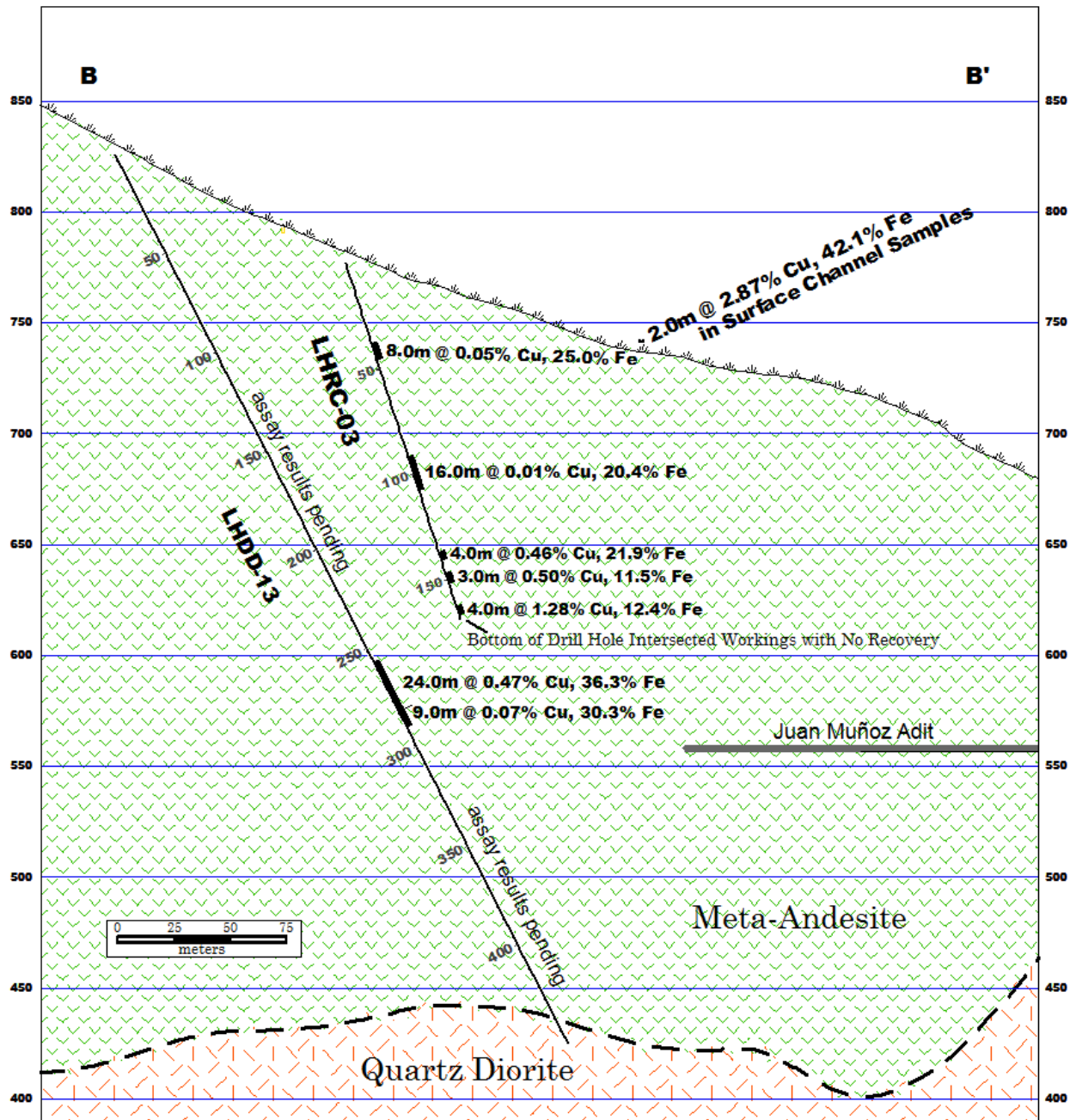
DRILL SECTION B-B'
