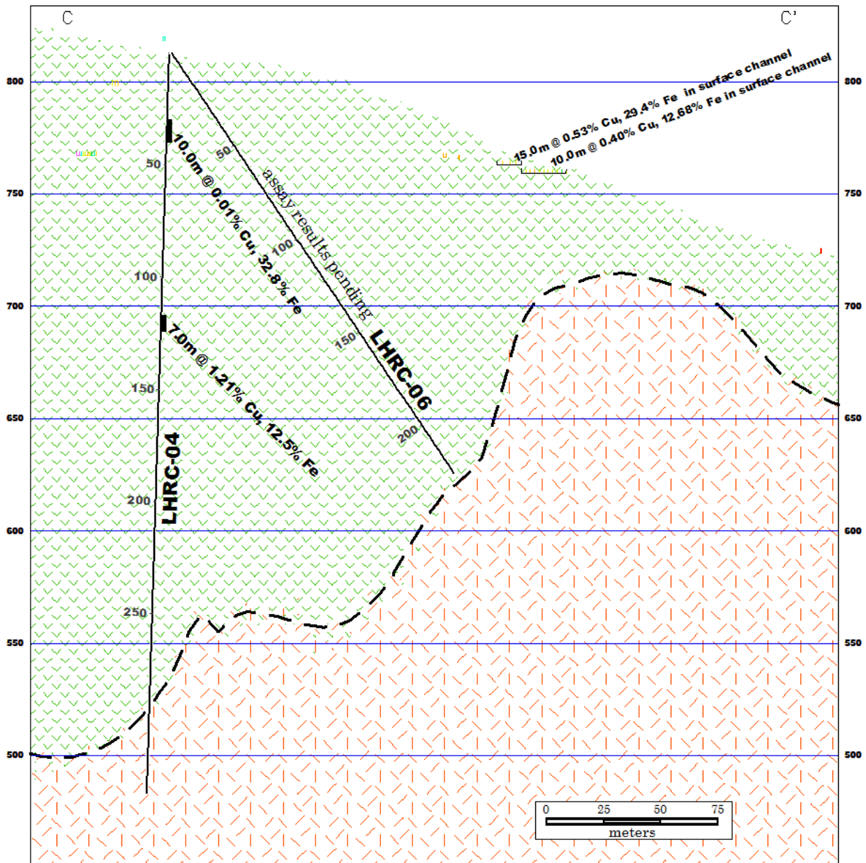
FIGURE 4 DRILL SECTION C-C'
