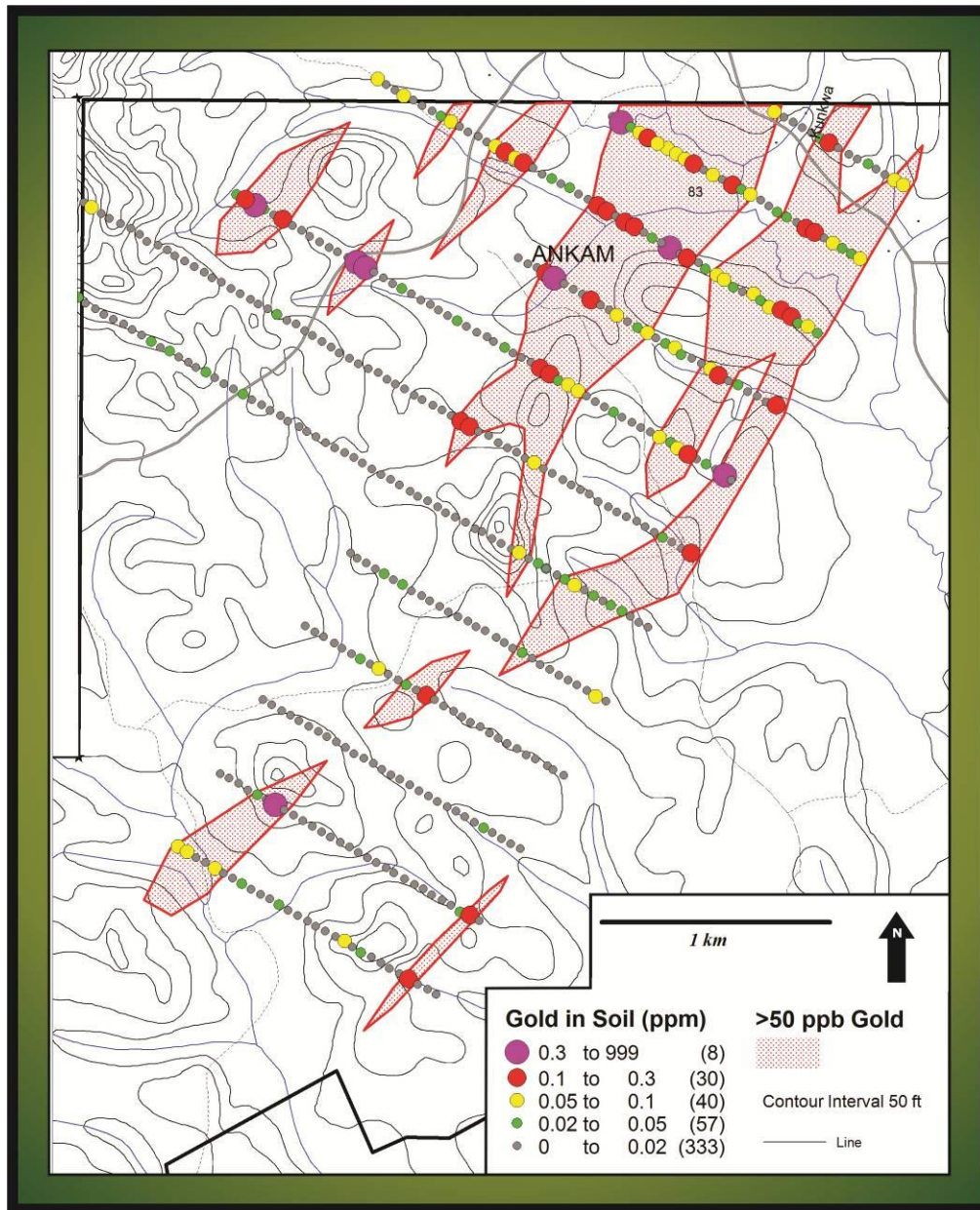
Figure 3. The newly discovered zone of gold surface samples, called Golden Reef East, is defined by samples containing gold in excess of 0.05 g/t gold (shown in red stippled pattern) over areas up to 3 km long and 0.6 km wide.
