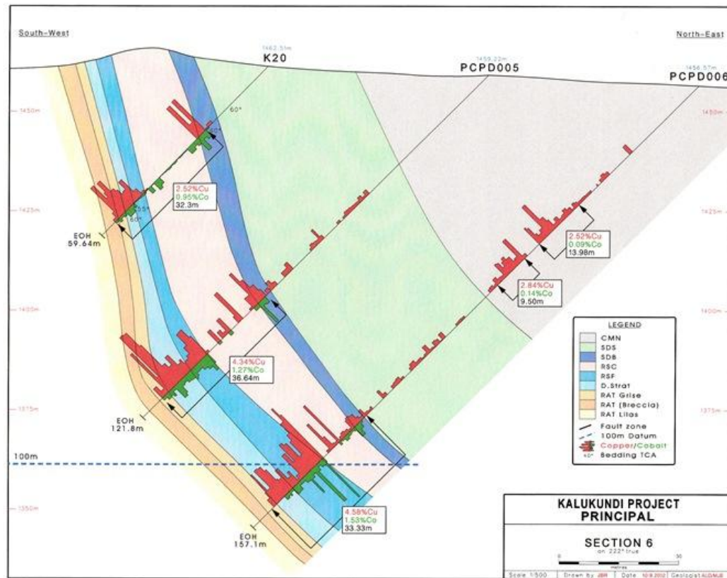
Figure 2. Section from the Principal Fragment midway on the grid (Figure 1), showing two recent intersections, PCPD005 and PCPD006 and indicating excellent continuity of the oxide mineralization in the Mines Series and oxide mineralisation in the hangingwall formations.
