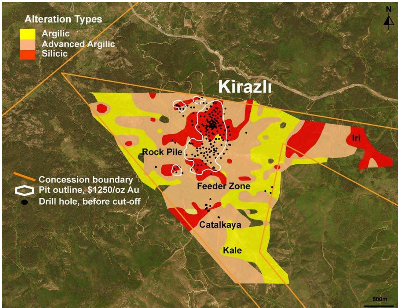
Figure 5: Kirazlı Project Alteration and Known Gold Occurrences
