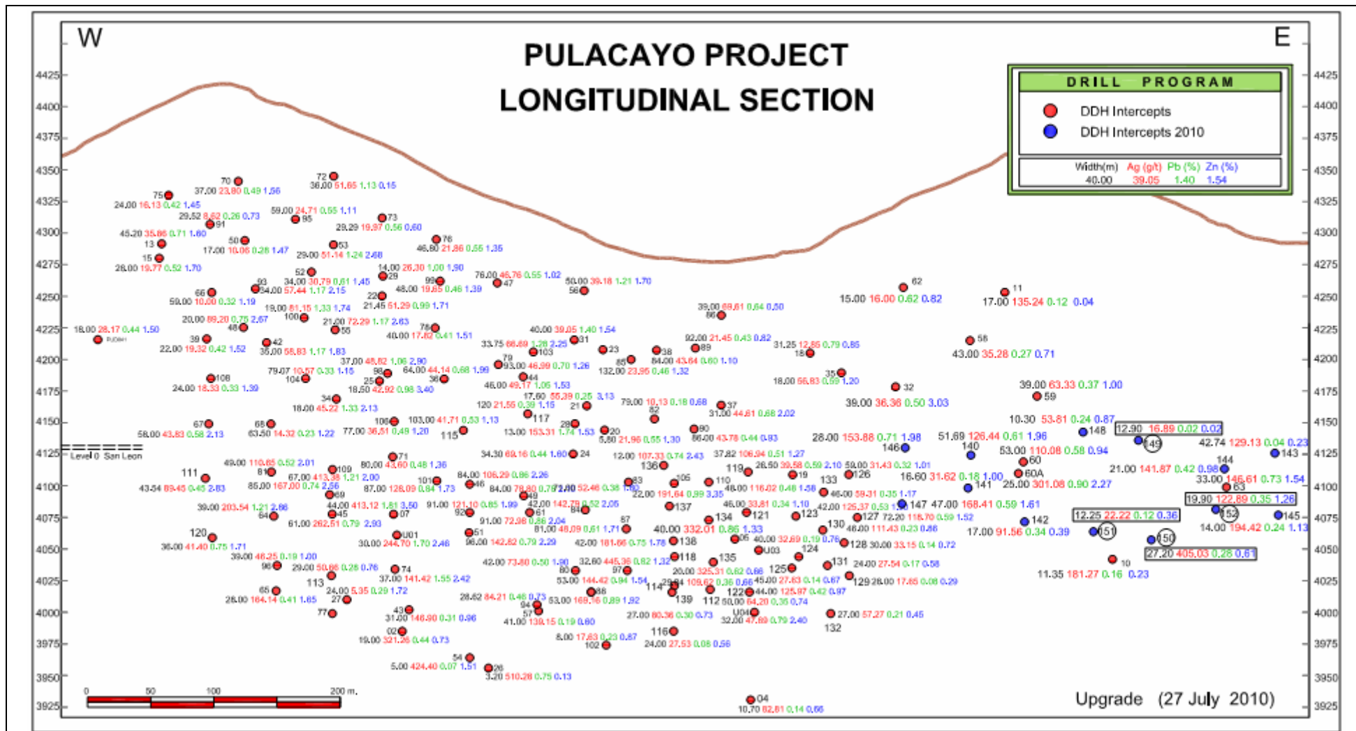
Figure 3: Pulacayo Deposit Vertical Longitudinal Sections
