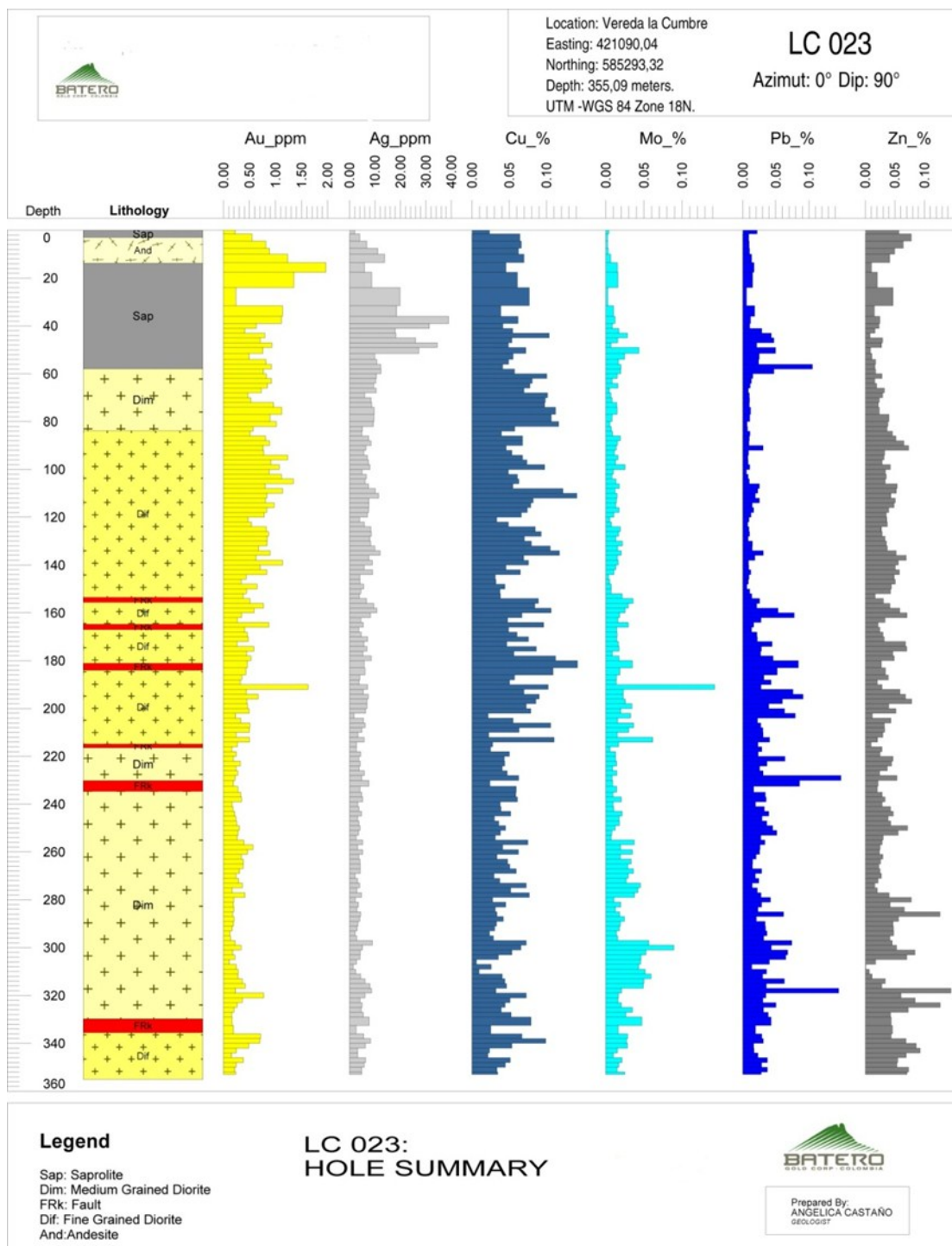
Figure 2 – Strip Log for Drill Hole LC 023
