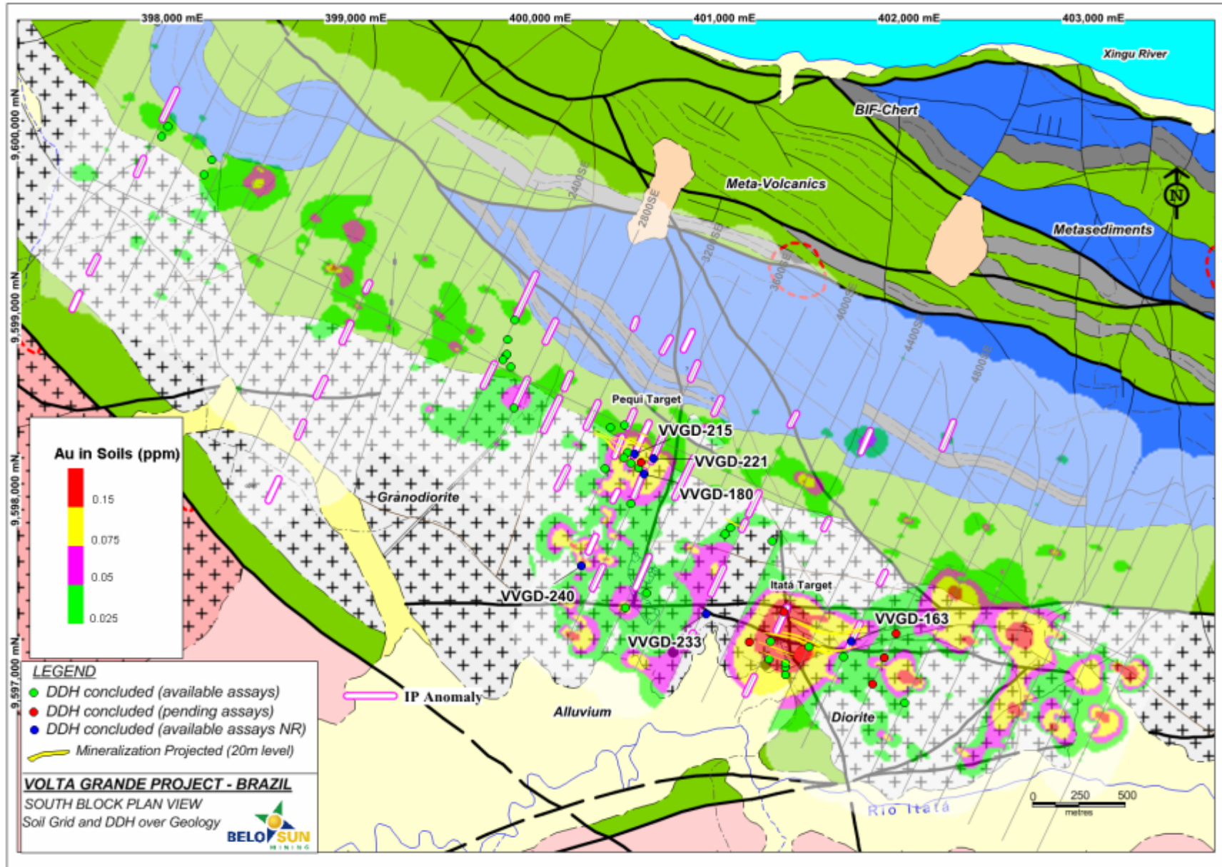
Figure 3 – South Block Geological Map
