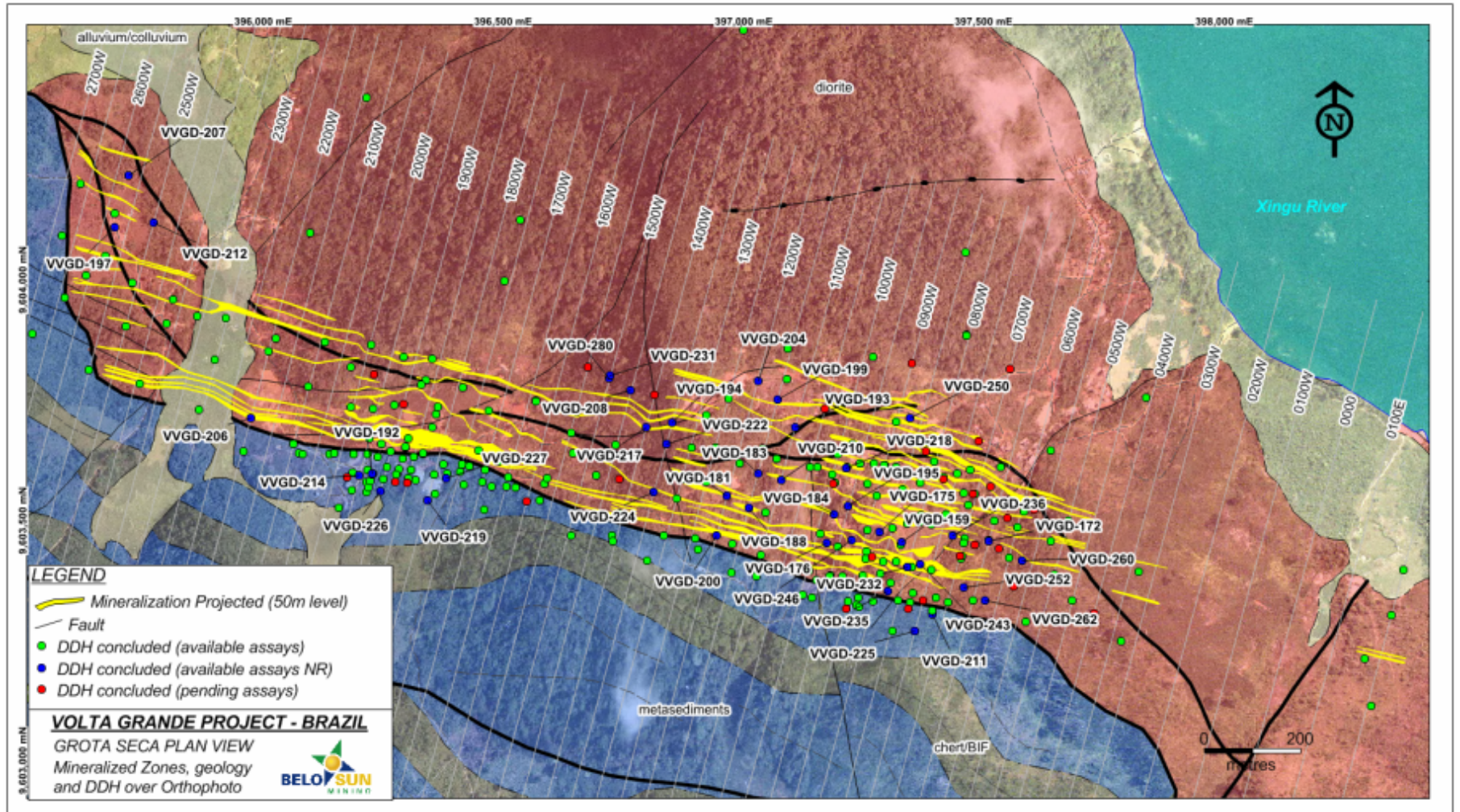
Figure 2 – Grota Seca Geological Map
