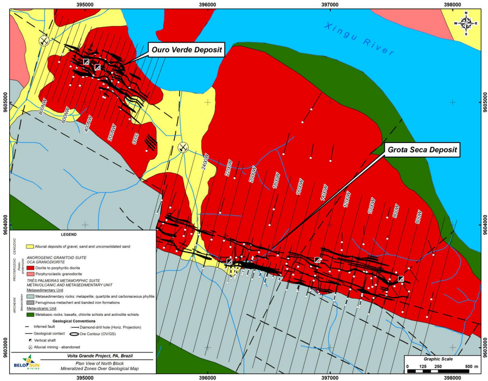
Figure 1 – Volta Grande Geological Map and main deposits location
