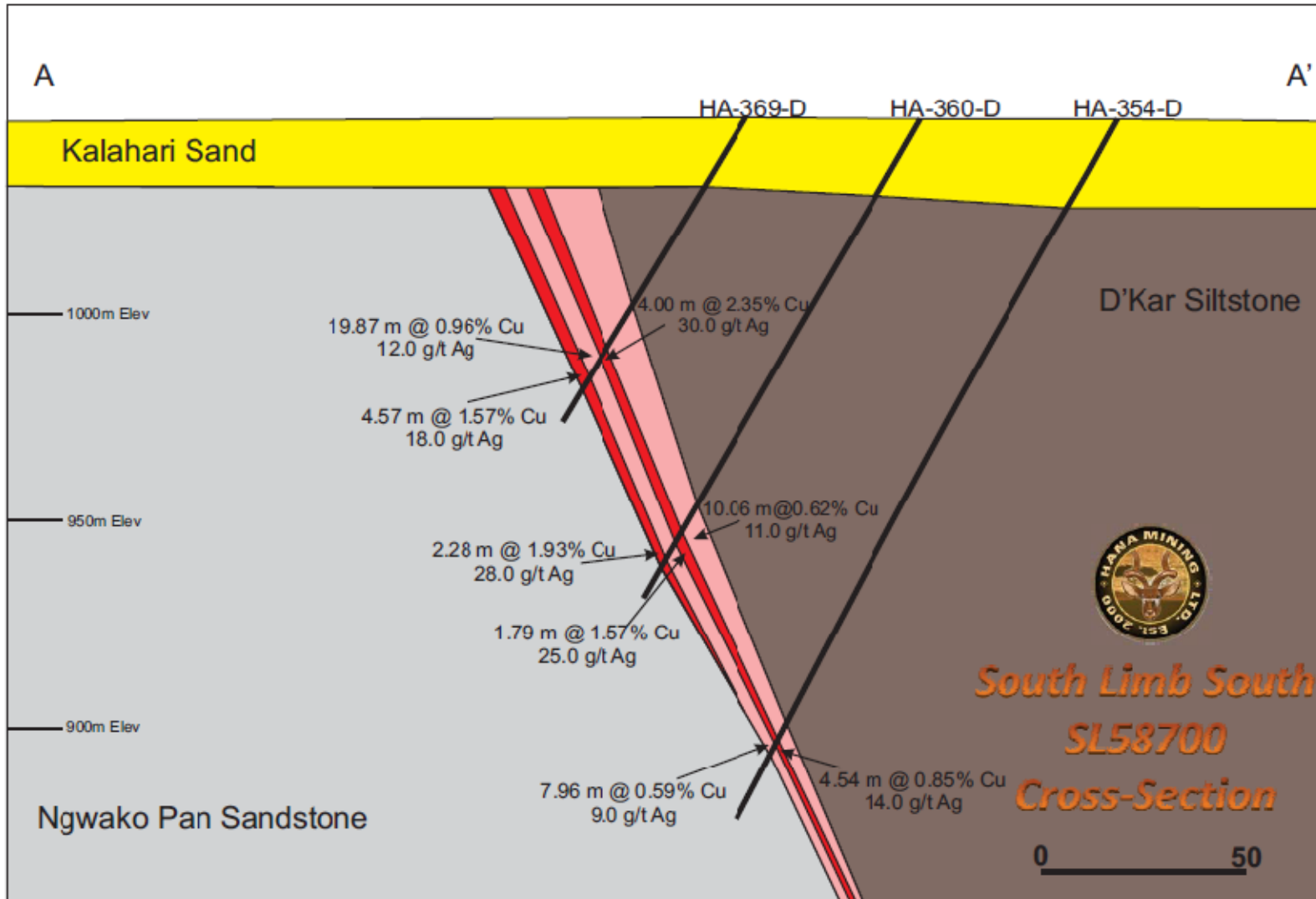
Figure 3: Cross-section through section 58700 (South Limb South)
