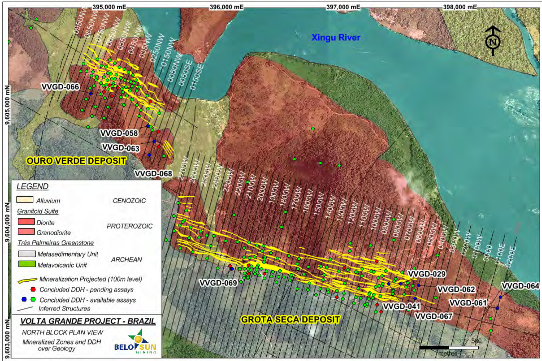
Figure 1 – Volta Grande Geological Map and main deposits location
