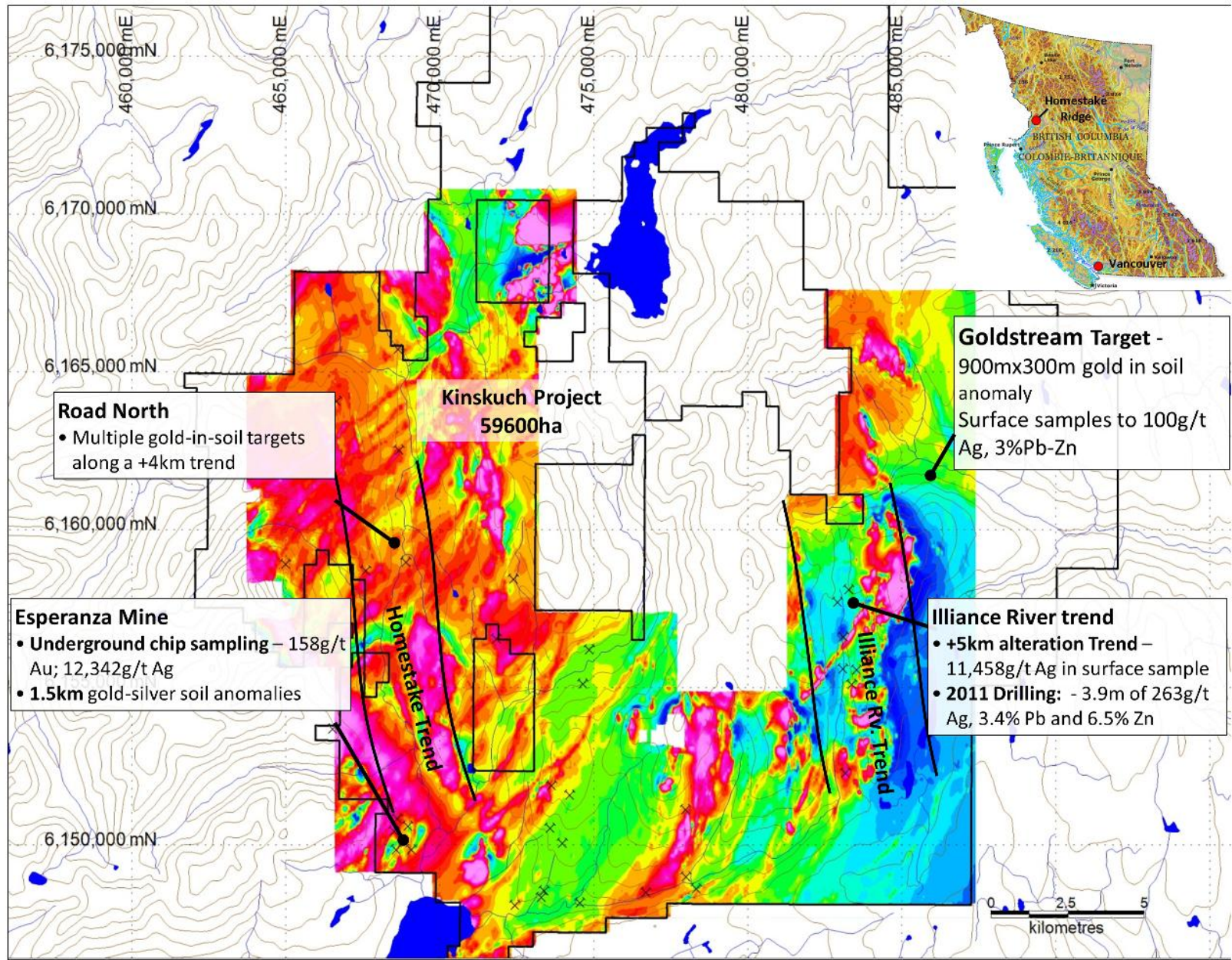
Figure 1: Residual Magnetic intensity map of the Kinskuch project, note the pronounced magnetic low along Illiance River trend
