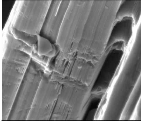
High magnification view revealing sharply defined edge of graphite crystal, with near perfect layering of graphene sheets. (65,000 X magnification)
