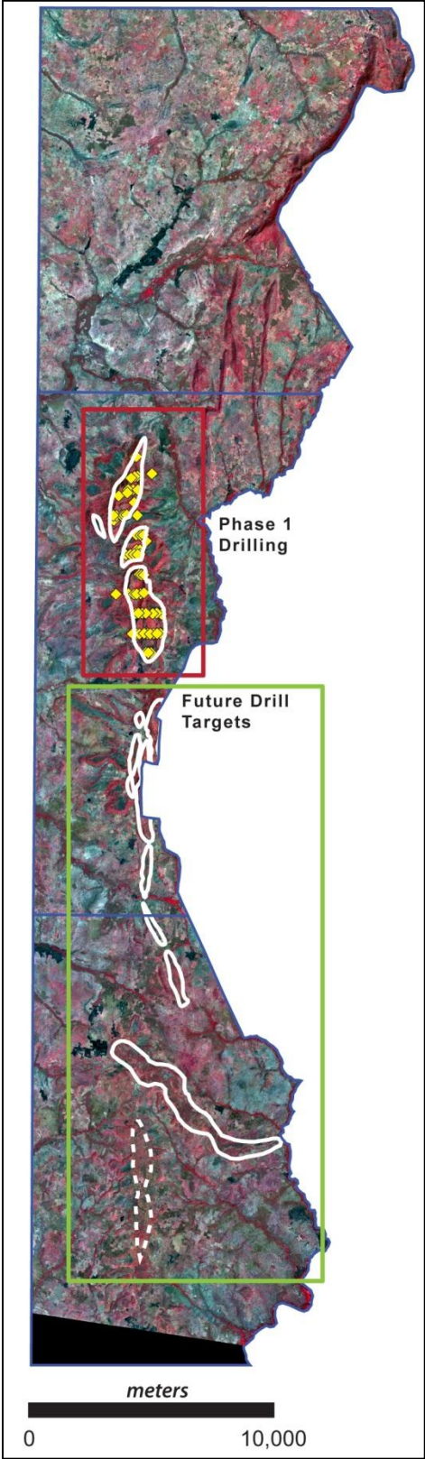
Figure 1: Satellite Image (Aster bands 3n-2-1) showing Phase I drill area and the area for future exploration. Interpreted areas of outcropping ironstone are outlined in white. Drillholes are shown as yellow symbols.
