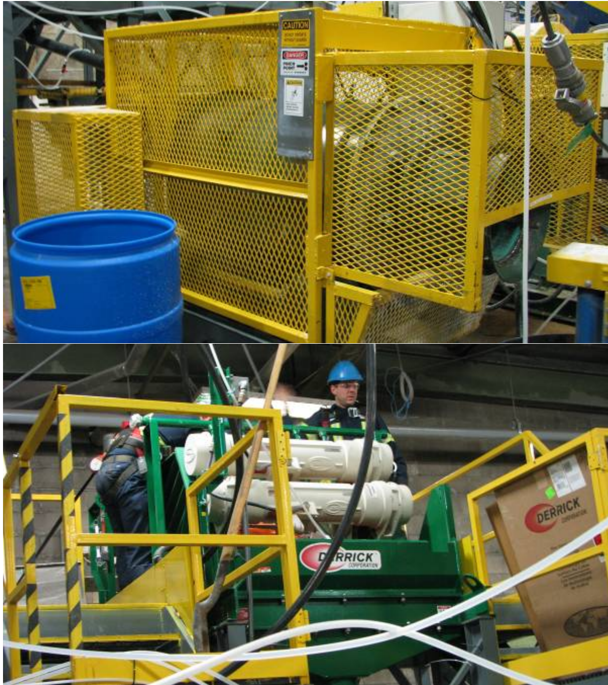
Figure 2 - Ball Mill & Derrick Screen. Overs from Derrick feed Ball Mill
