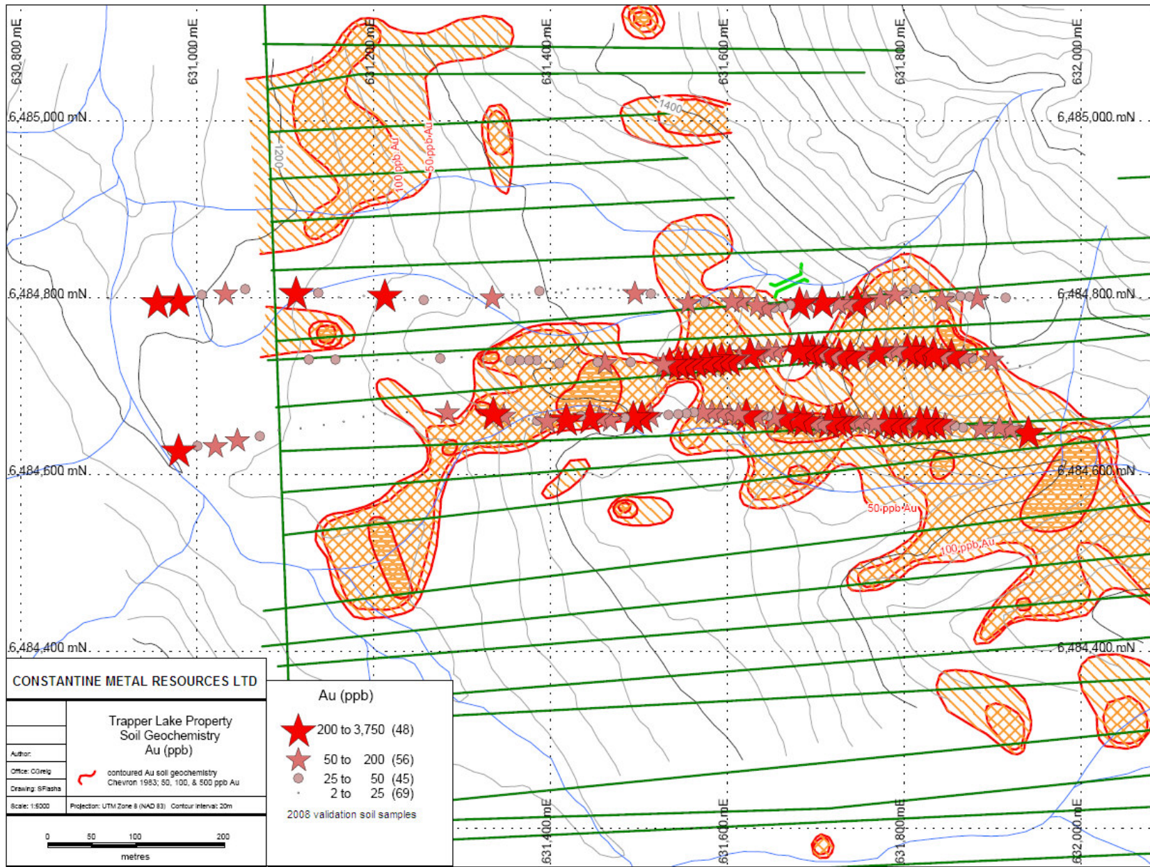
Figure 2. Trapper Lake property soil anomaly map, including 1983 Chevron gold-in-soil contours overlain by 2008 validation soil samples (three lines).
