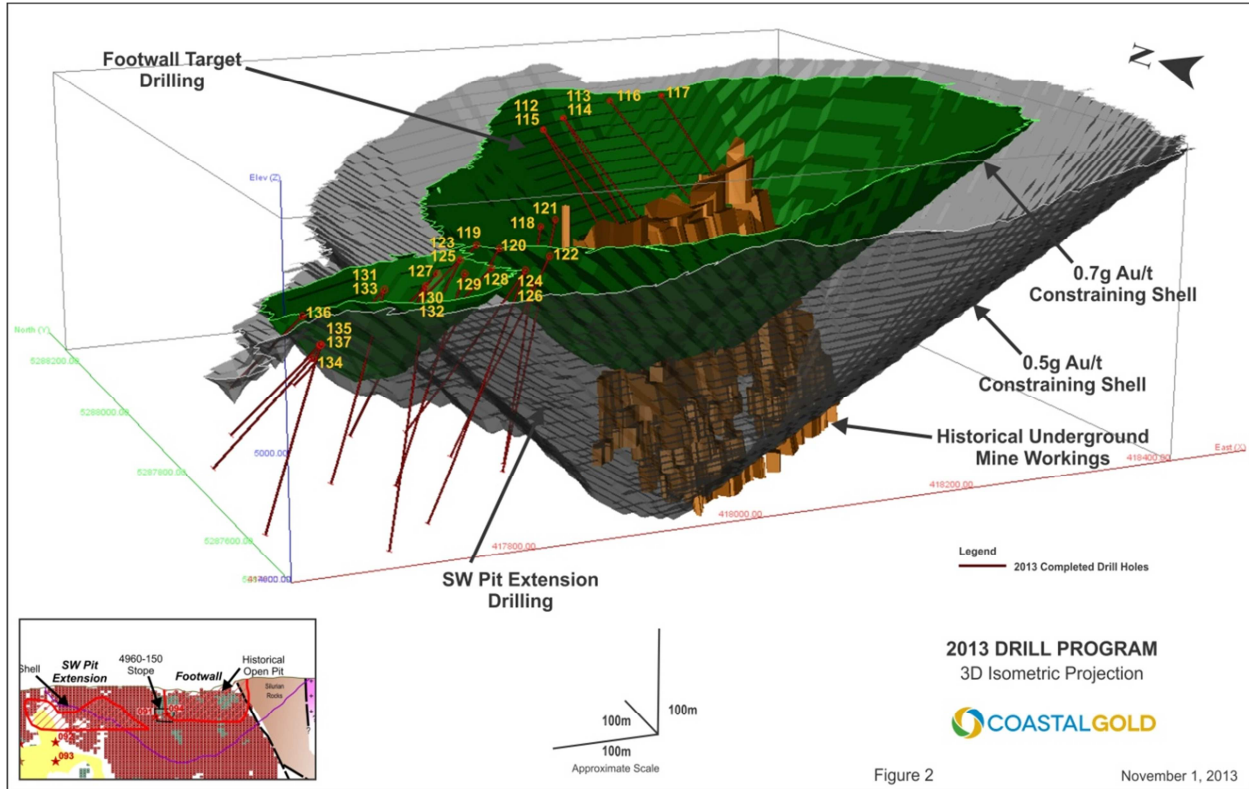
FIGURE 2: 3D ISOMETRIC PROJECTIONS
