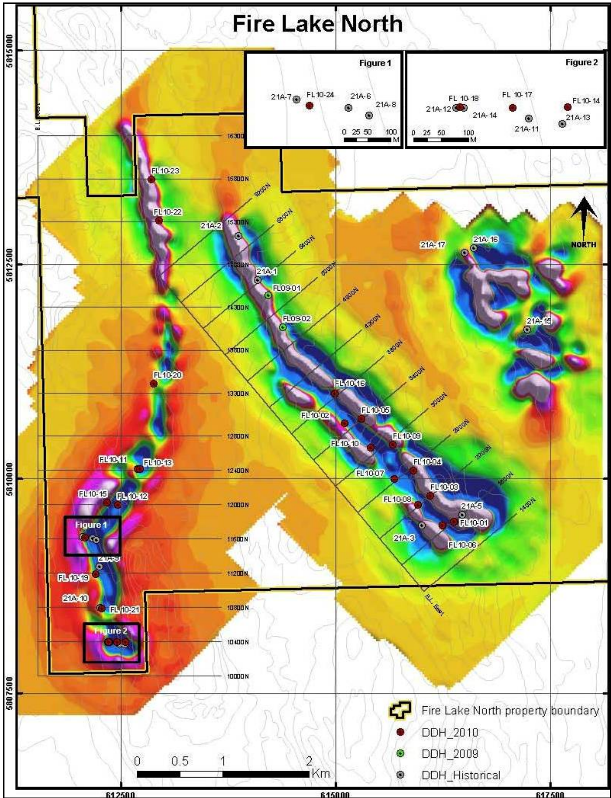
Fire Lake North Claim Block, Fermont Iron Property – Location Map of the 2010 Winter Diamond Drilling Campaign, with reference to diamond drill holes FLN-10-01 and 06 along the southern tip (bottom right) of the East Limb Iron Formation proximal to historic drill holes 21A-3 and 21A-5.
