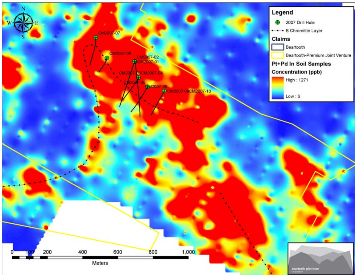
Figure 1 Map illustrating the large Pt+Pd soil geochemical anomaly associated with the CM Zone of PGM mineralization, and the locations of the 2007 drill holes in the Chrome Mountain area.
