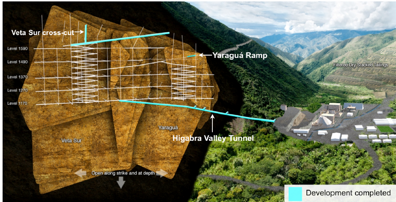
Figure 1: Buriticá Preliminary Development Plan*
