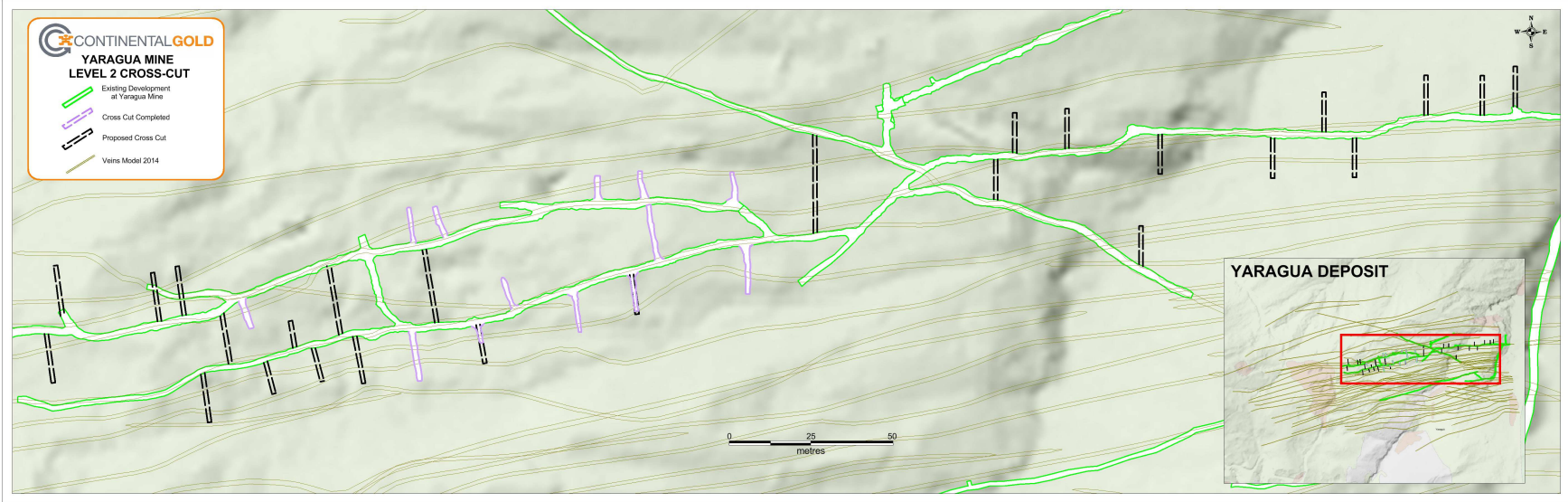
Figure 4: Yaraguá Mine – Level 2 Cross-cut
