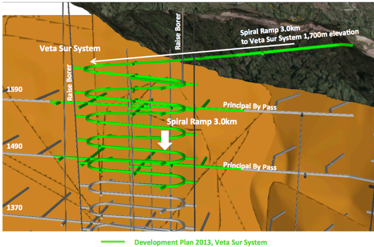
Figure 2: Three-kilometre Ramp Accessing Veta Sur System
