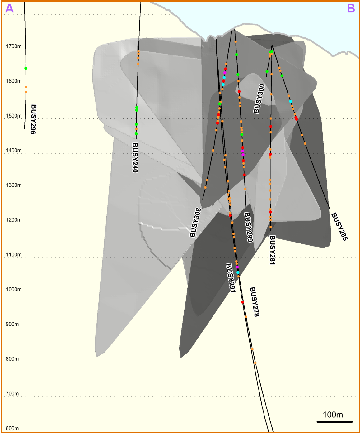
Figure 2 – Longitudinal section of Veta Sur drilling highlights and the current mineral resource model
