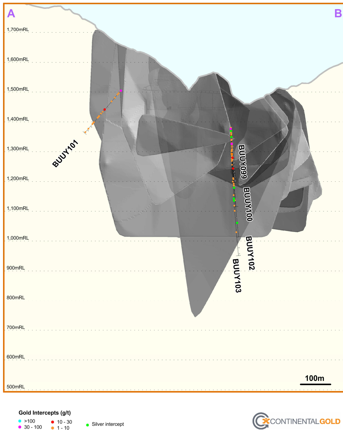
Figure 3 – Long Section of the Yaraguá Vein System, Showing New Drilling Highlights, Against the October 2012 Mineral Resource Envelope
