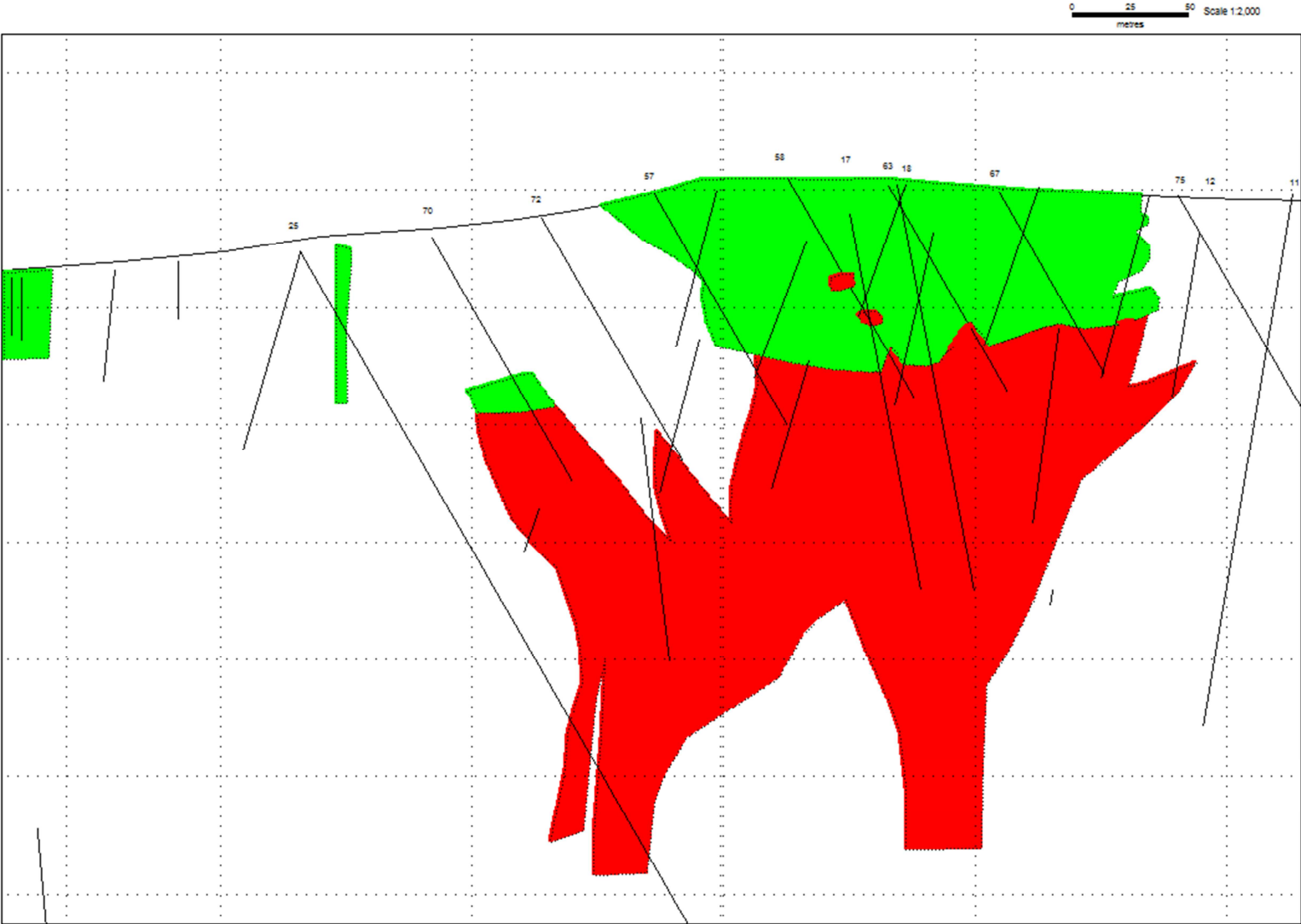
Figure 2; Berta Sur Cross Section, looking NE. Copper oxide mineralization shown in green, sulphide mineralization in red.
