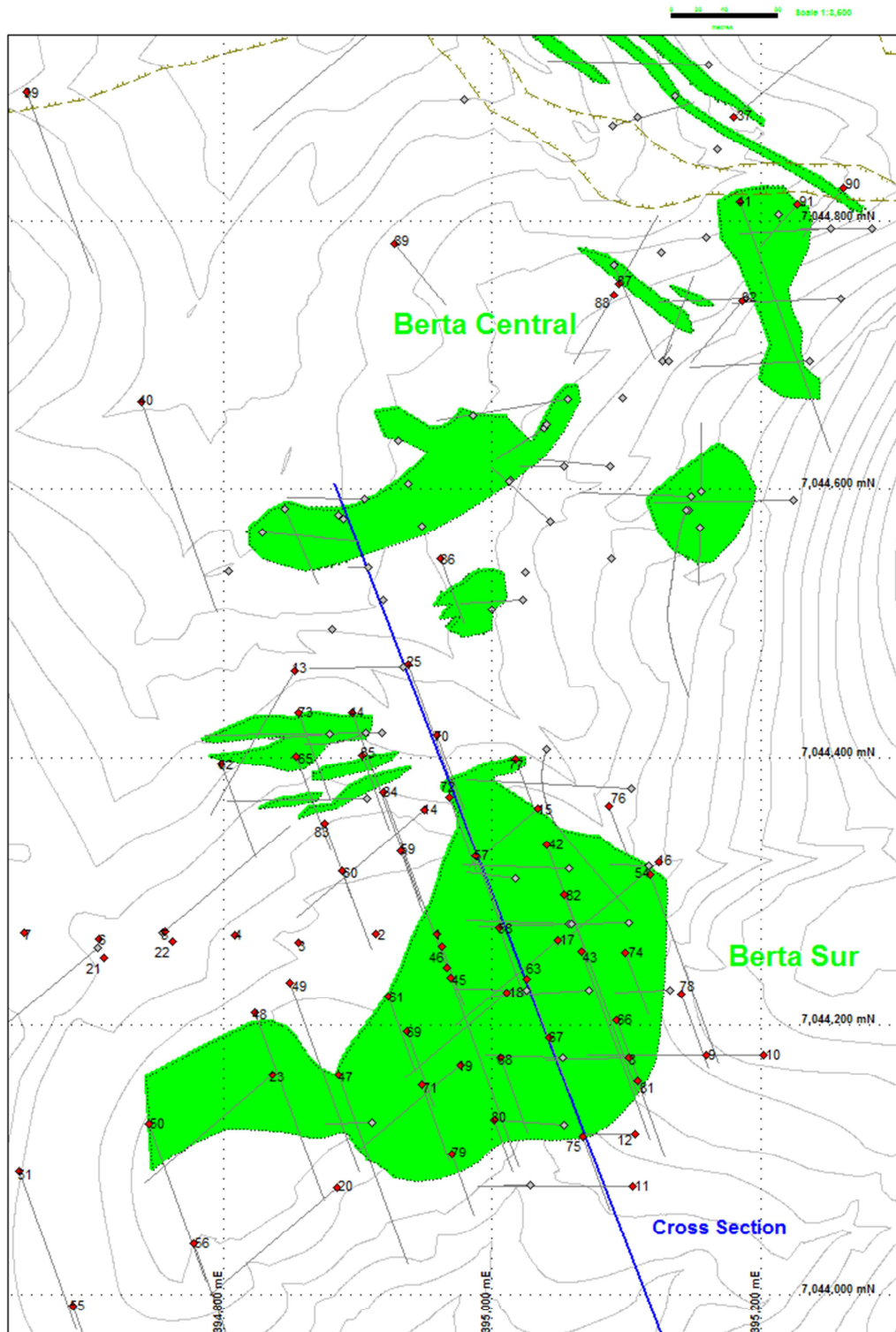
Figure 1; Berta Sur and Central areas. Drill tested copper oxide mineralization shown in green, Coro RC hole collars in red, pre-2012 holes in grey.
