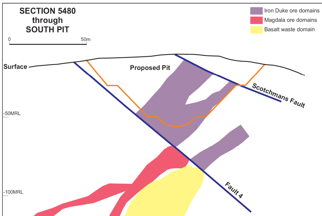
Figure 2: South Pit Cross Section
