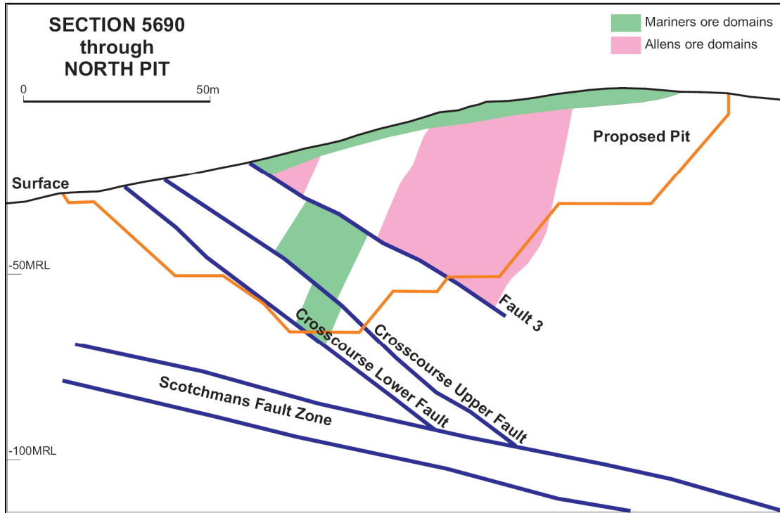
Figure 1: North Pit Cross Section
