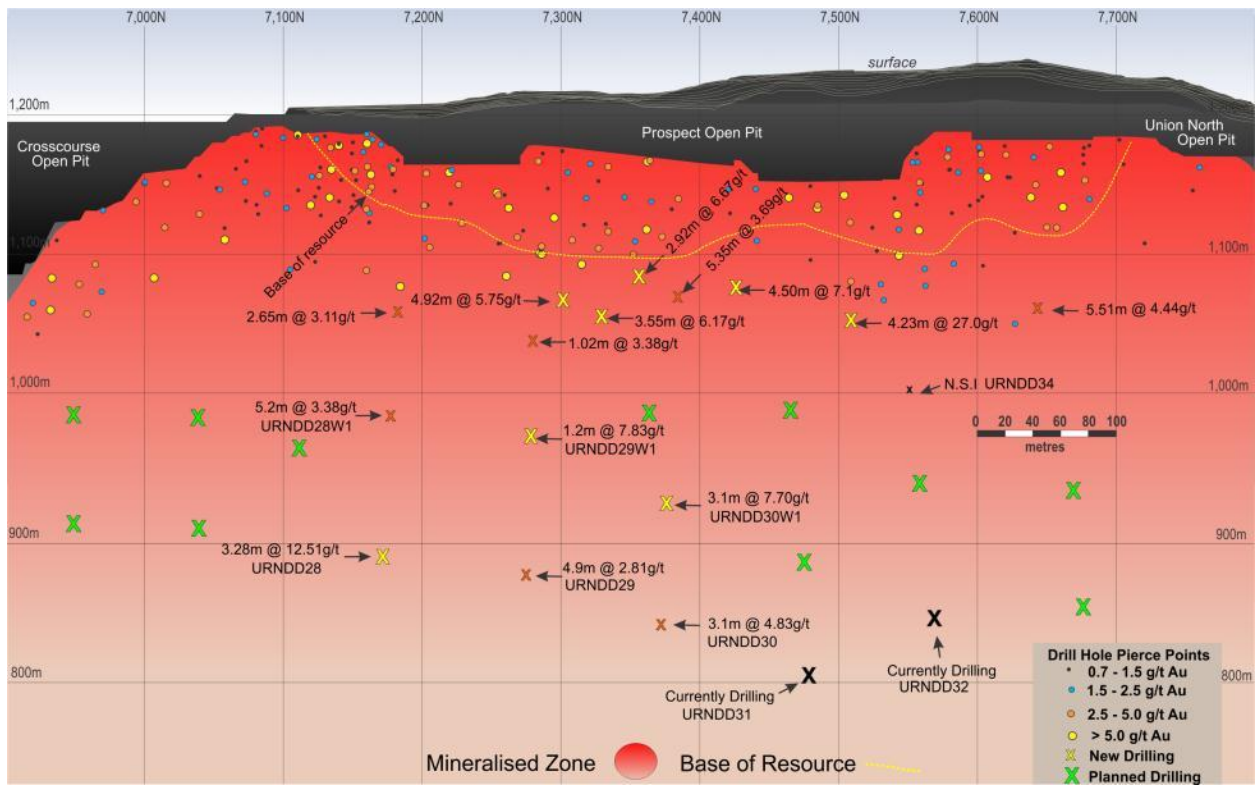
Figure 7: Prospect Long Section showing latest results
