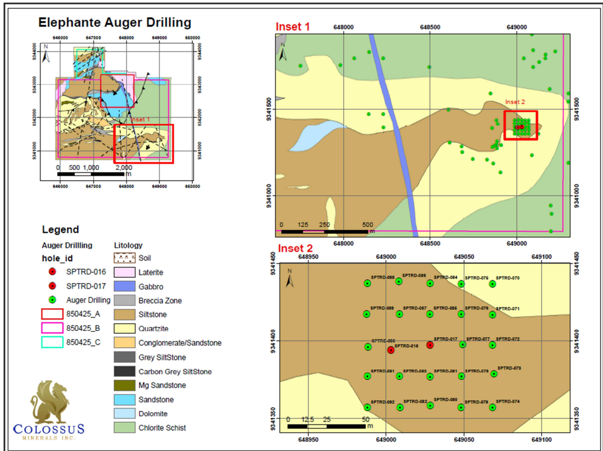
Figure 1: Auger drill hole location plan for the Elefante Area.
